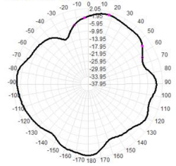
Total(H-XY), Max= 0.42dBi, CirD=11.98
