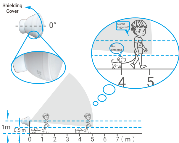
Fig. 1 Side view of the detection range
