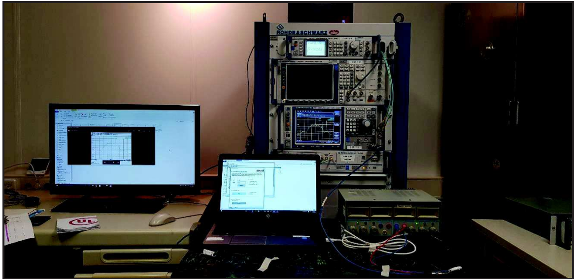
Photo 5 : Conducted Measurements
