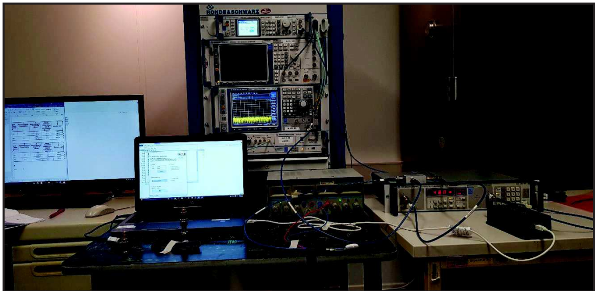
Photo 6 : Conducted Measurements
