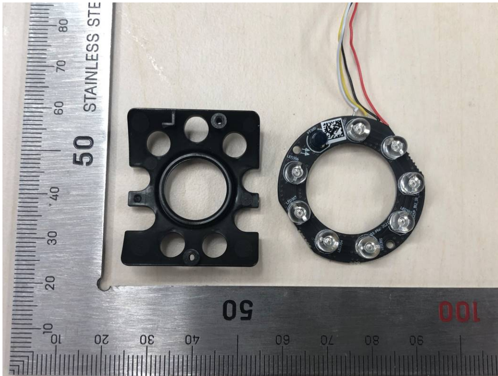
Fig. 15. Camera PCB view -8
