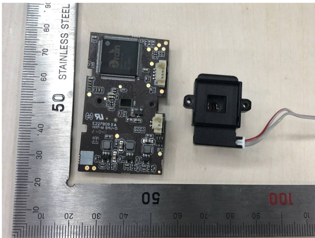
Fig. 14. Camera PCB view -7
