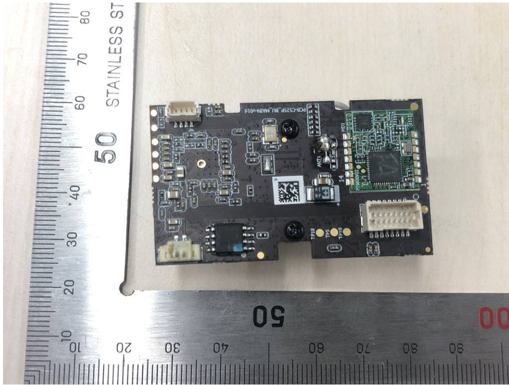
Fig. 13. Camera PCB view -6
