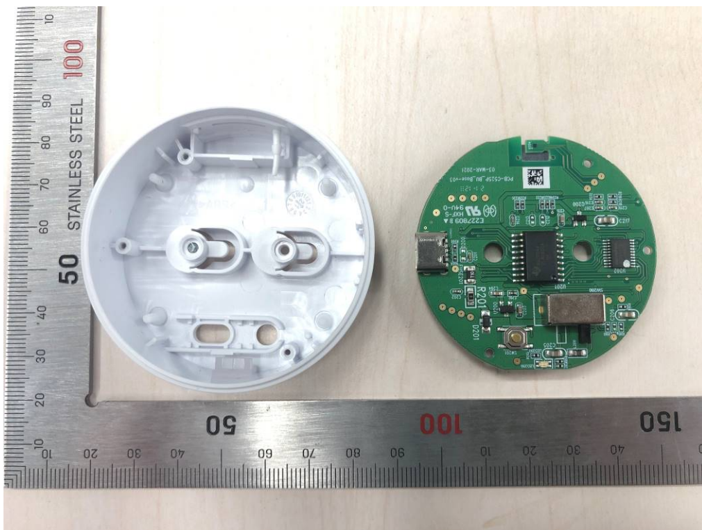
Fig. 2. Camera internal view -2
