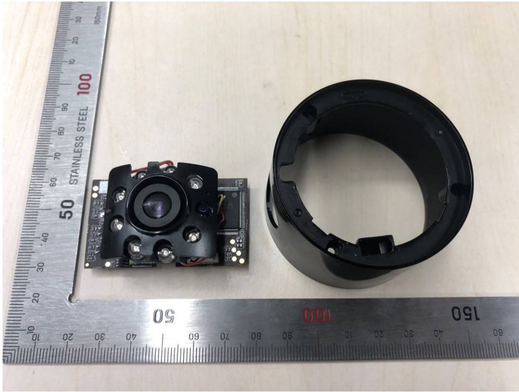
Fig. 7. Camera internal view -8
