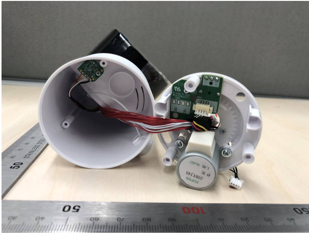
Fig. 3. Camera internal view -4
