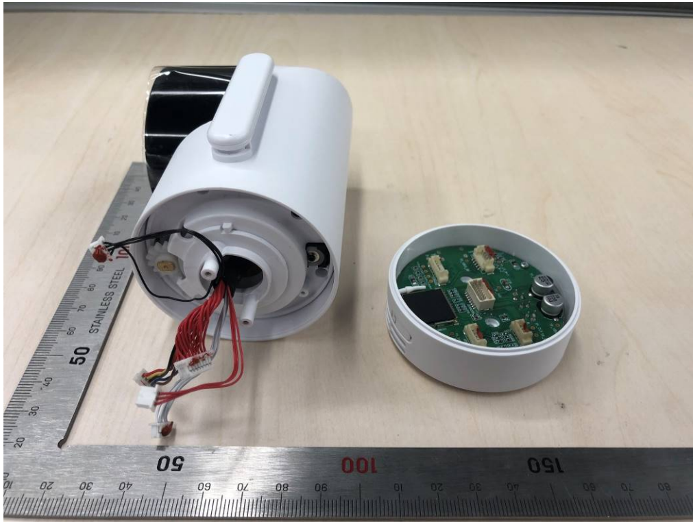
Fig. 1. Camera internal view -1
