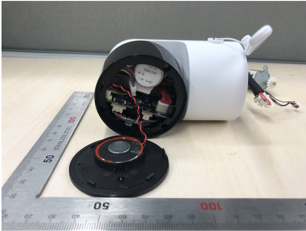
Fig. 5. Camera internal view -6
