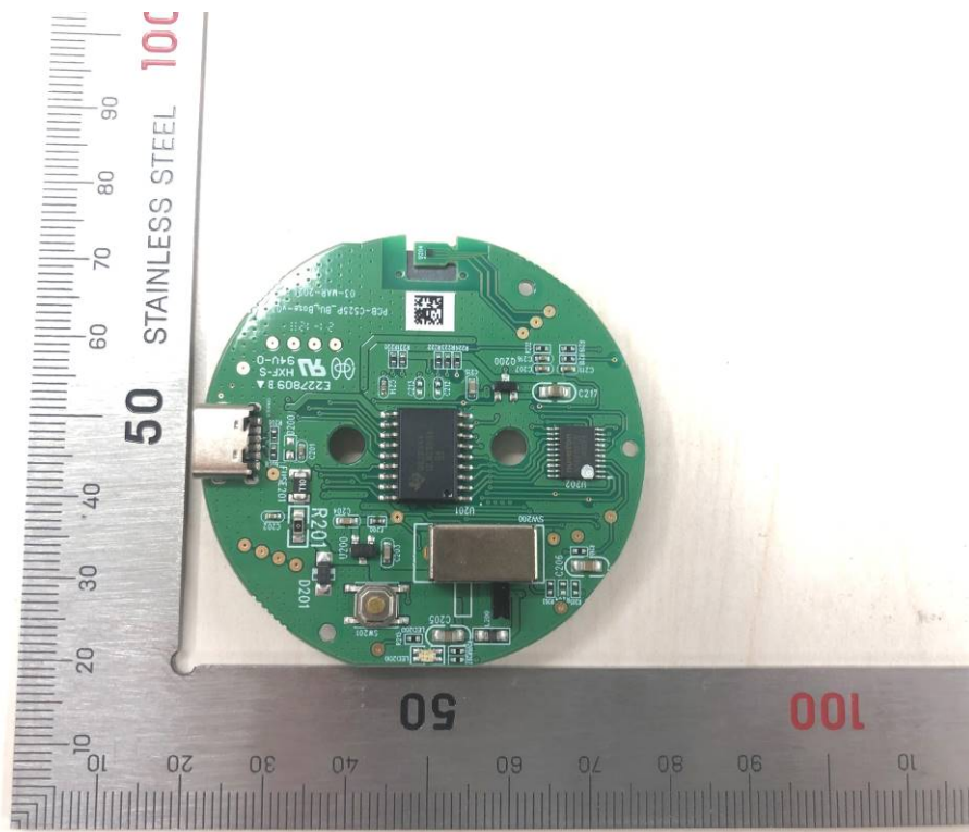
Fig. 8. Camera PCB view -1
