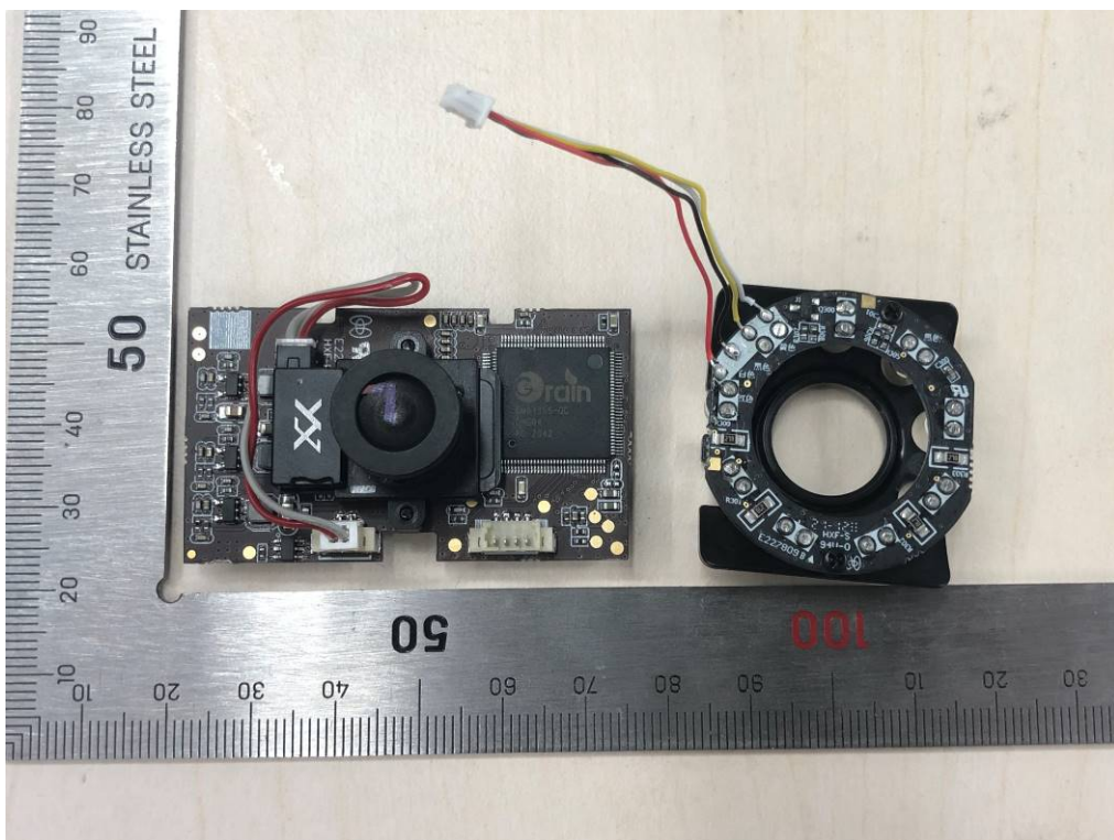
Fig. 12. Camera PCB view -5
