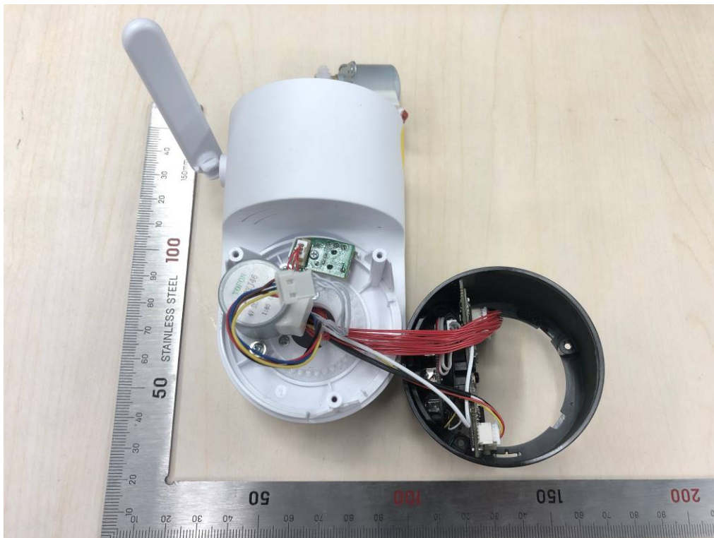
Fig. 6. Camera internal view -7
