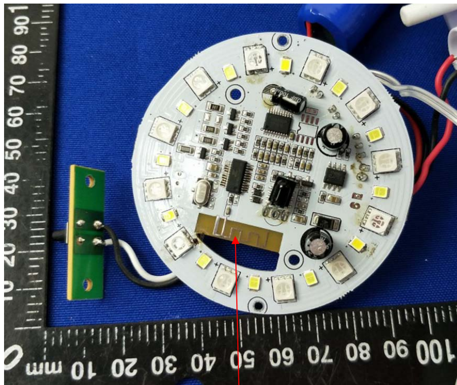
BT Antenna
