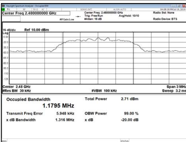
Channel 78 (2480MHz)
