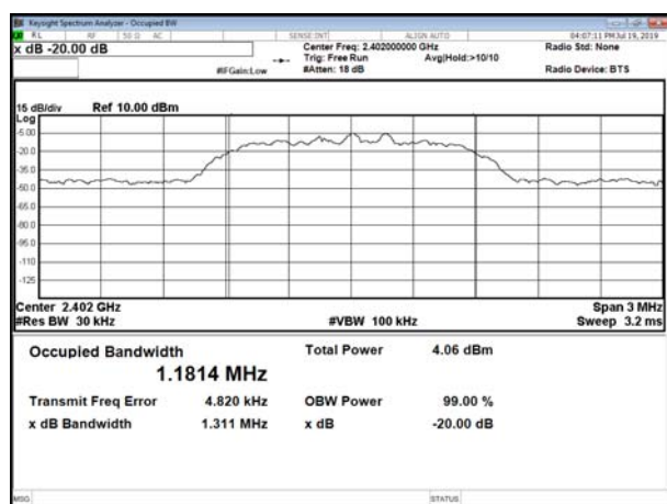
Channel 00 (2402MHz)
