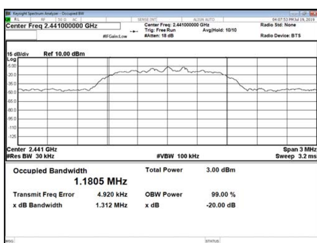
Channel 39 (2441MHz)
