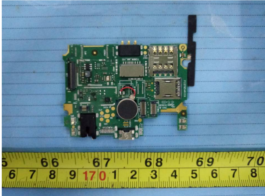
EUT – Main Board Bottom Shielding off View
