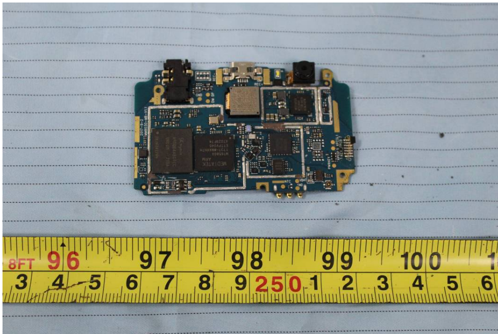
EUT – Main Board 1 Bottom Shieding off View
