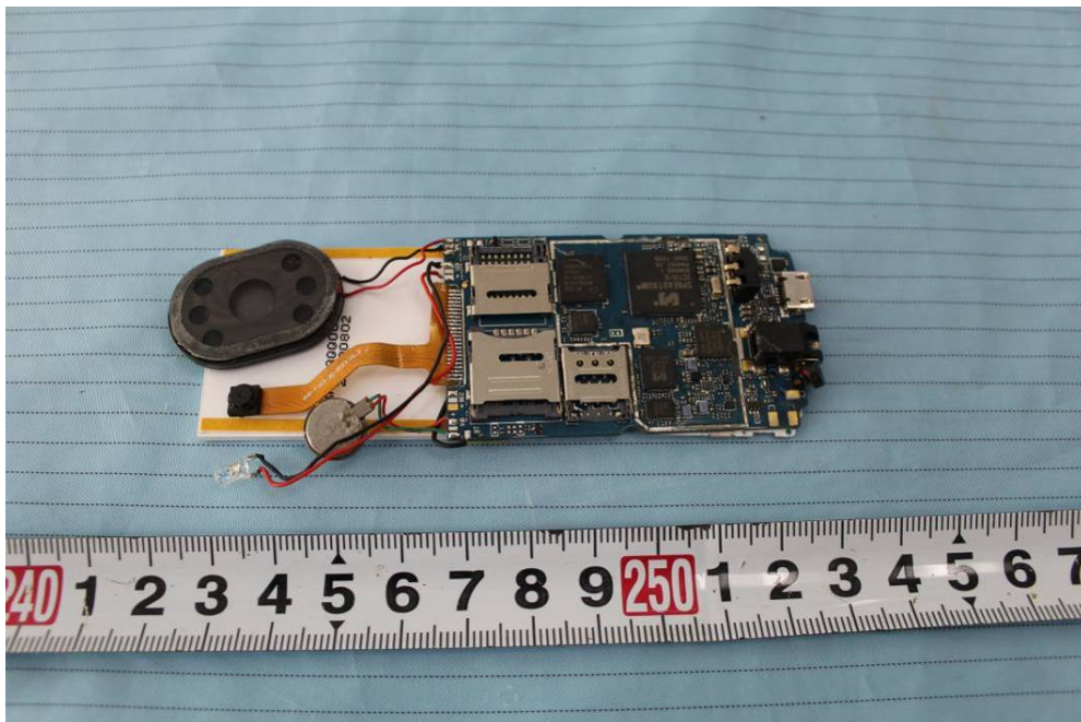
EUT –Main Board Bottom Shilding off View
