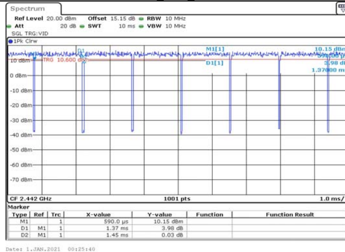
11N20SISO_Ant1_2442
