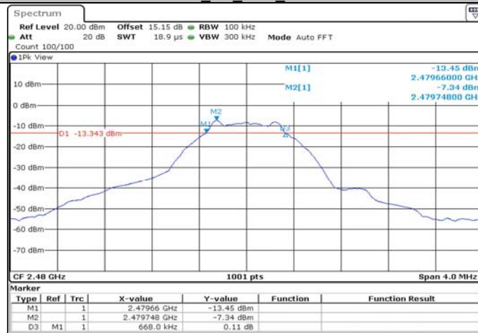
BLE_1M_Ant1_2480
