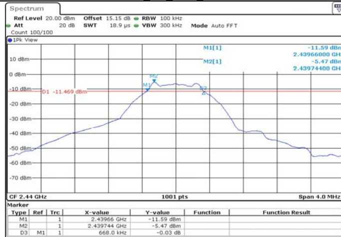
BLE_1M_Ant1_2440
