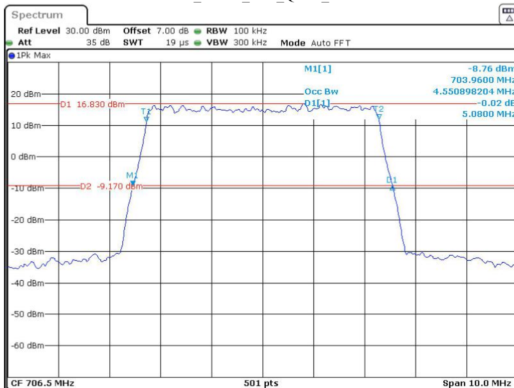
Band 17_5 MHz_Low_QPSK_RB25#0
