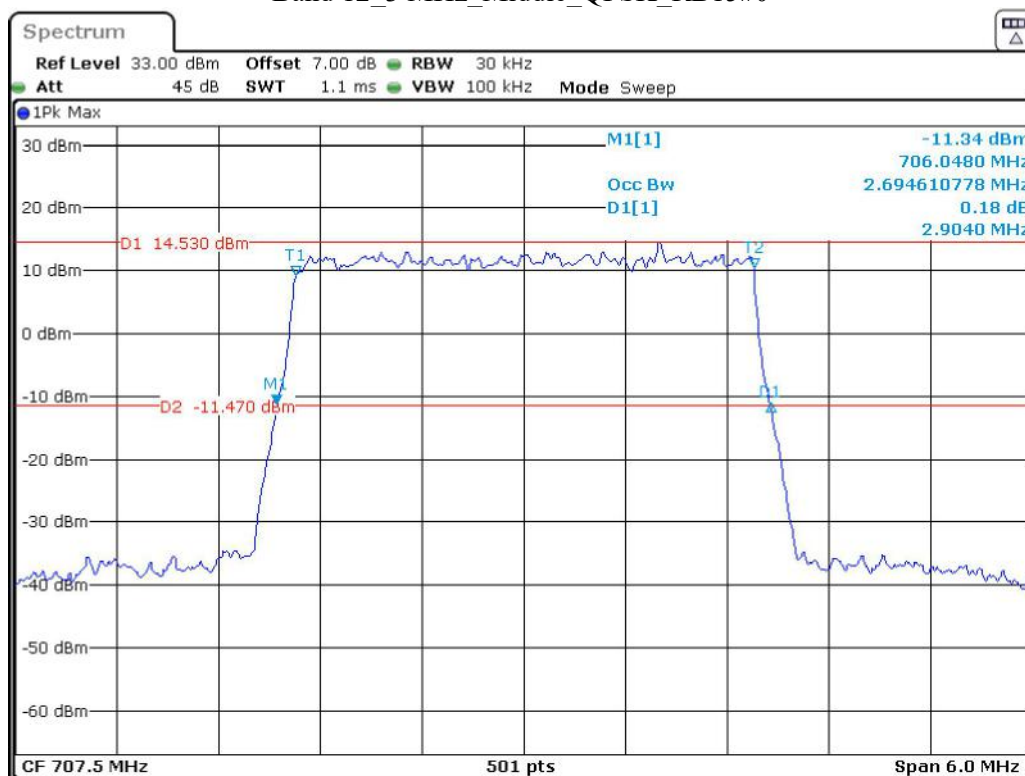
Band 12_3 MHz_Middle_QPSK_RB15#0
