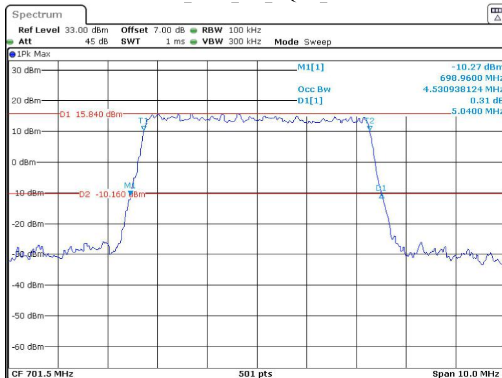
Band 12_5 MHz_Low_16QAM_RB25#0
