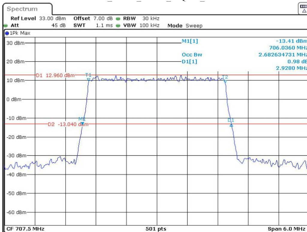
Band 12_3 MHz_Middle_16QAM_RB15#0
