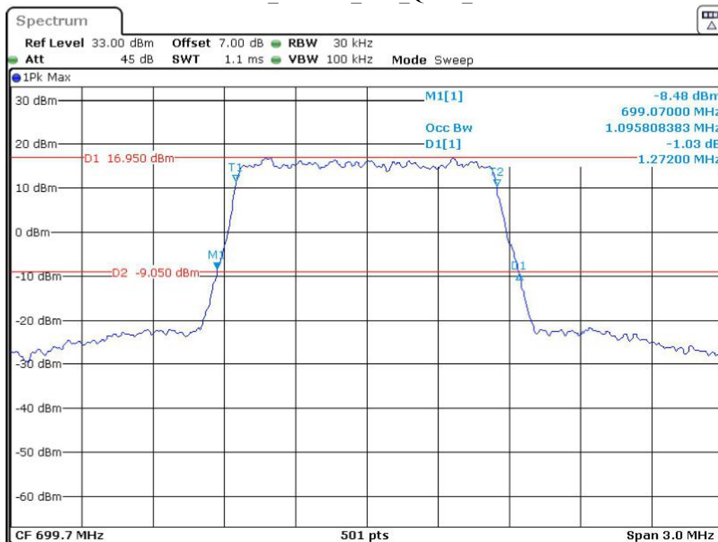
Band 12_1.4 MHz_Low_QPSK_RB6#0
