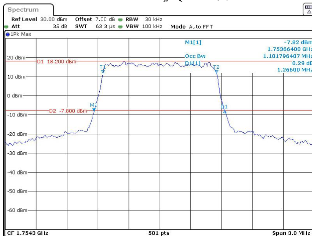
Band 4_1.4 MHz_High_QPSK_RB6#0
