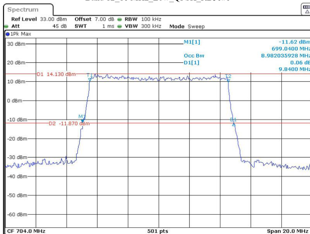
Band 12_10 MHz_Low_QPSK_RB50#0
