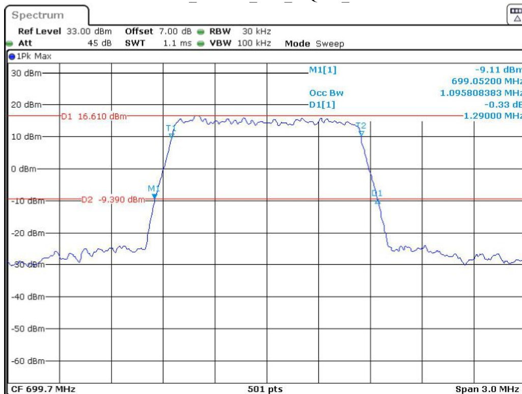
Band 12_1.4 MHz_Low_16QAM_RB6#0
