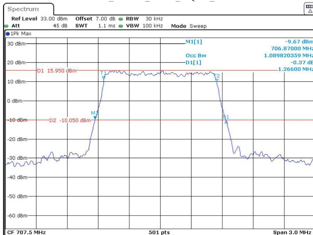
Band 12_1.4 MHz_Middle_16QAM_RB6#0
