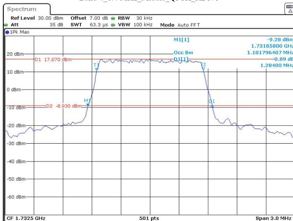
Band 4_1.4 MHz_Middle_QPSK_RB6#0
