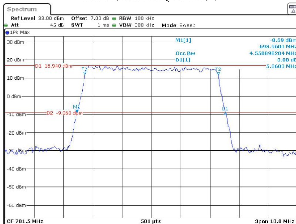
Band 12_5 MHz_Low_QPSK_RB25#0
