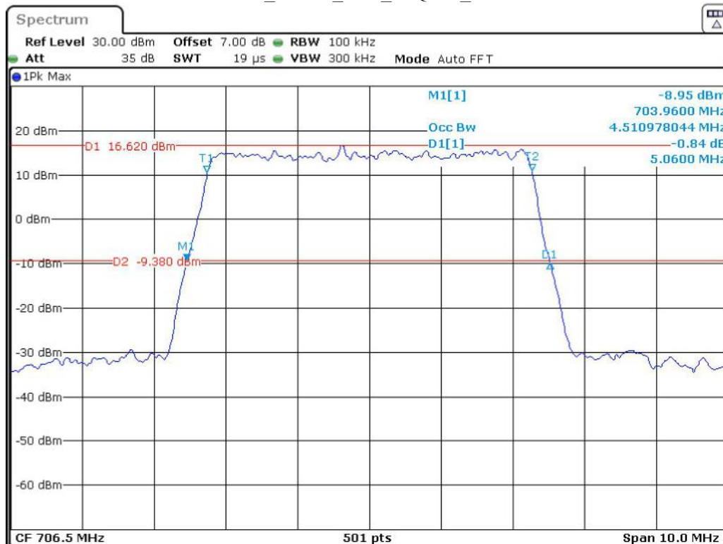
Band 17_5 MHz_Low_16QAM_RB25#0
