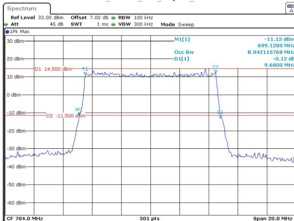
Band 12_10 MHz_Low_16QAM_RB50#0
