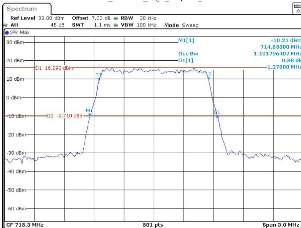
Band 12_1.4 MHz_High_16QAM_RB6#0
