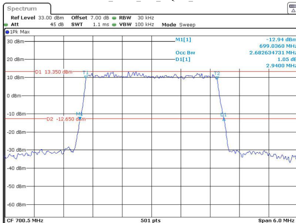
Band 12_3 MHz_Low_16QAM_RB15#0
