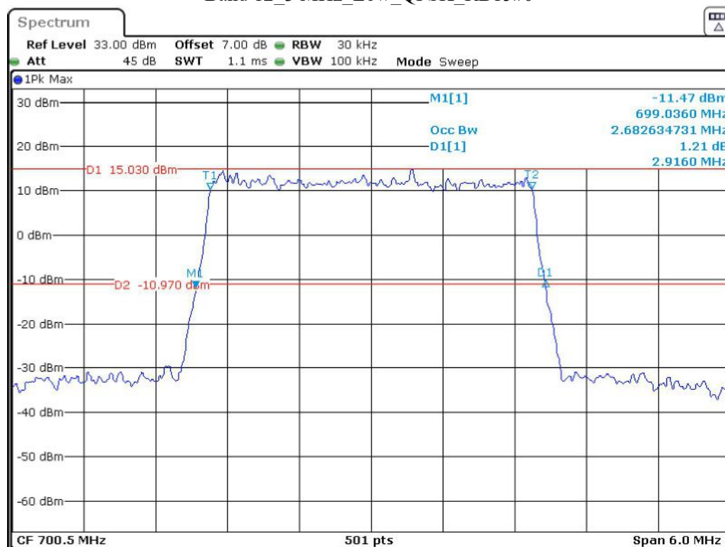
Band 12_3 MHz_Low_QPSK_RB15#0
