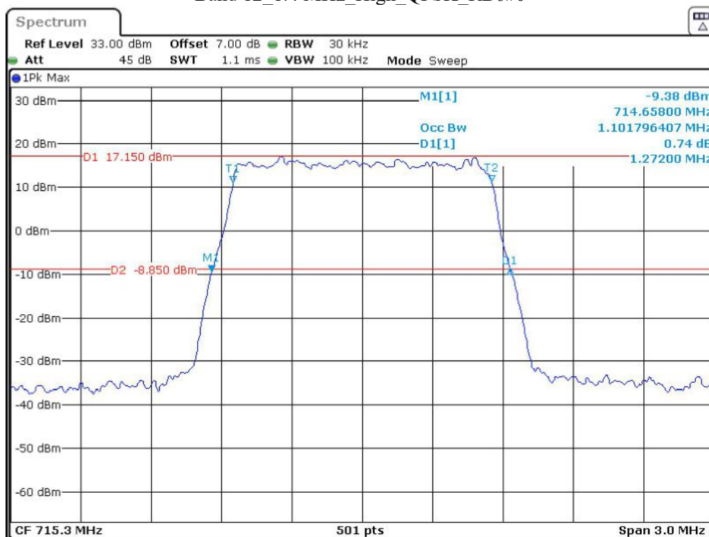
Band 12_1.4 MHz_High_QPSK_RB6#0
