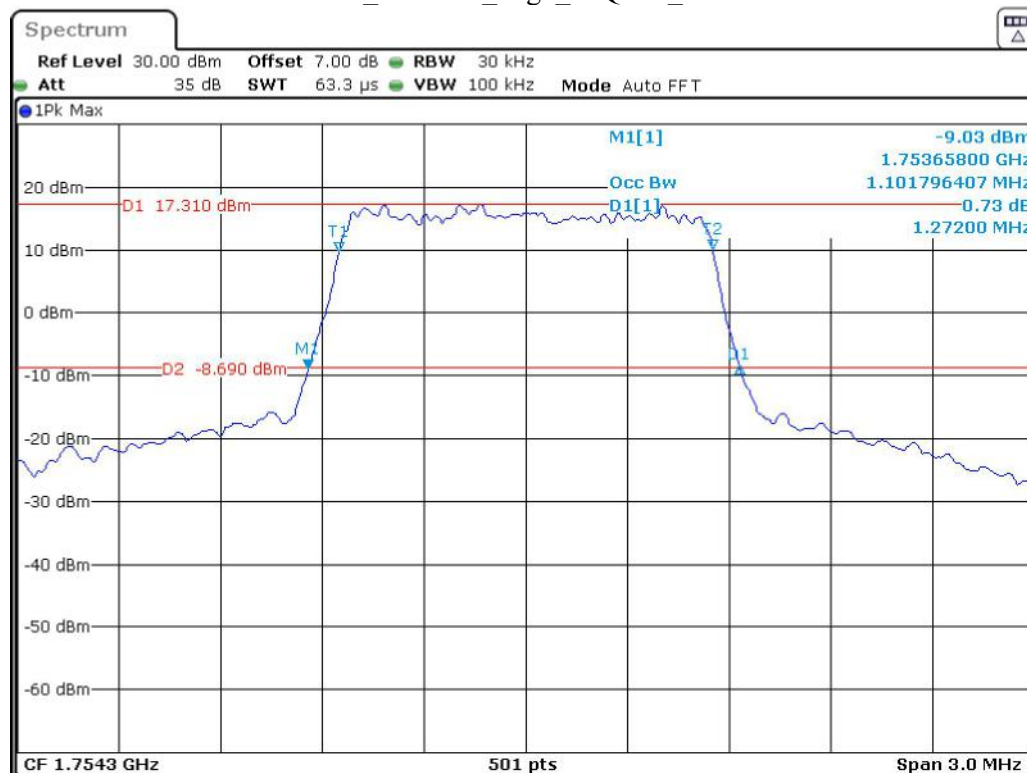
Band 4_1.4 MHz_High_16QAM_RB6#0
