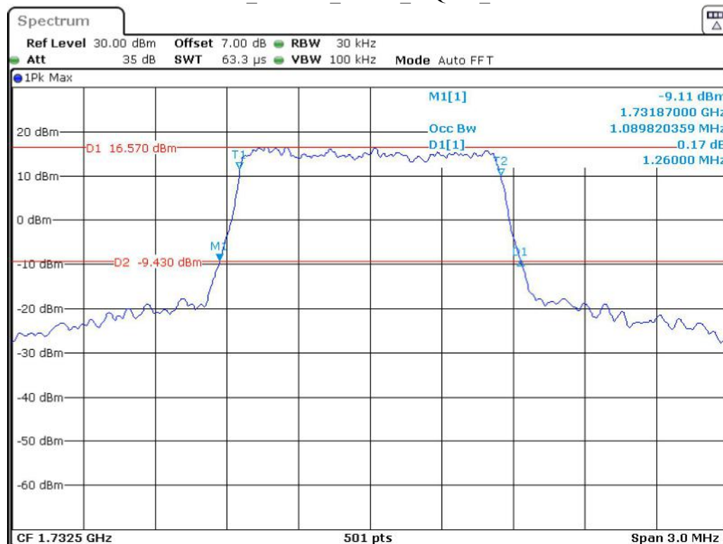
Band 4_1.4 MHz_Middle_16QAM_RB6#0
