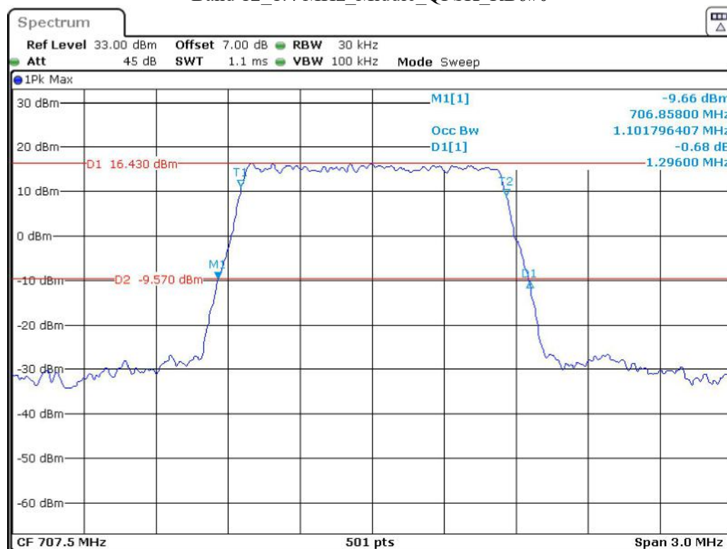
Band 12_1.4 MHz_Middle_QPSK_RB6#0
