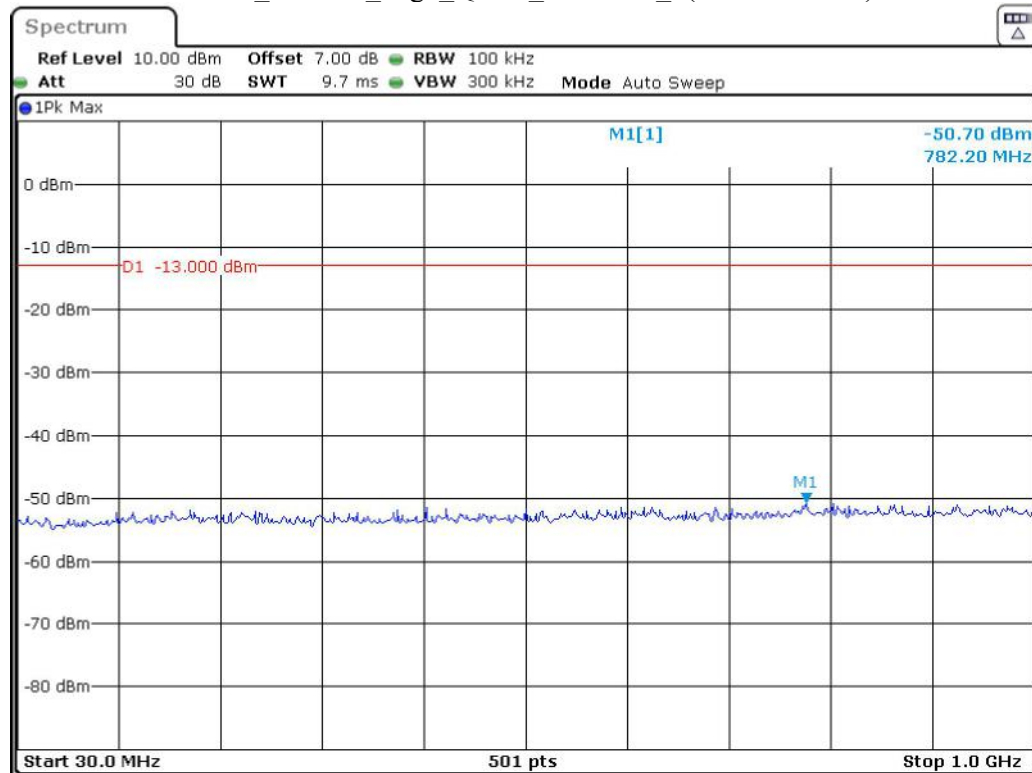
Band 4_20 MHz_High_QPSK_RB100#0_1(30MHz-1GHz)
