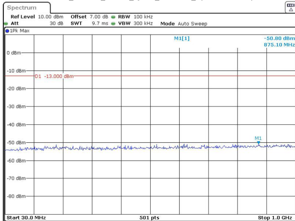
Band 4_20 MHz_Middle_QPSK_RB100#0_1(30MHz-1GHz)
