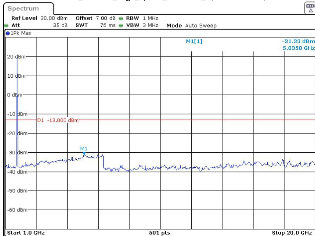
Band 4_20 MHz_High_QPSK_RB100#0_2(1GHz-20GHz)
