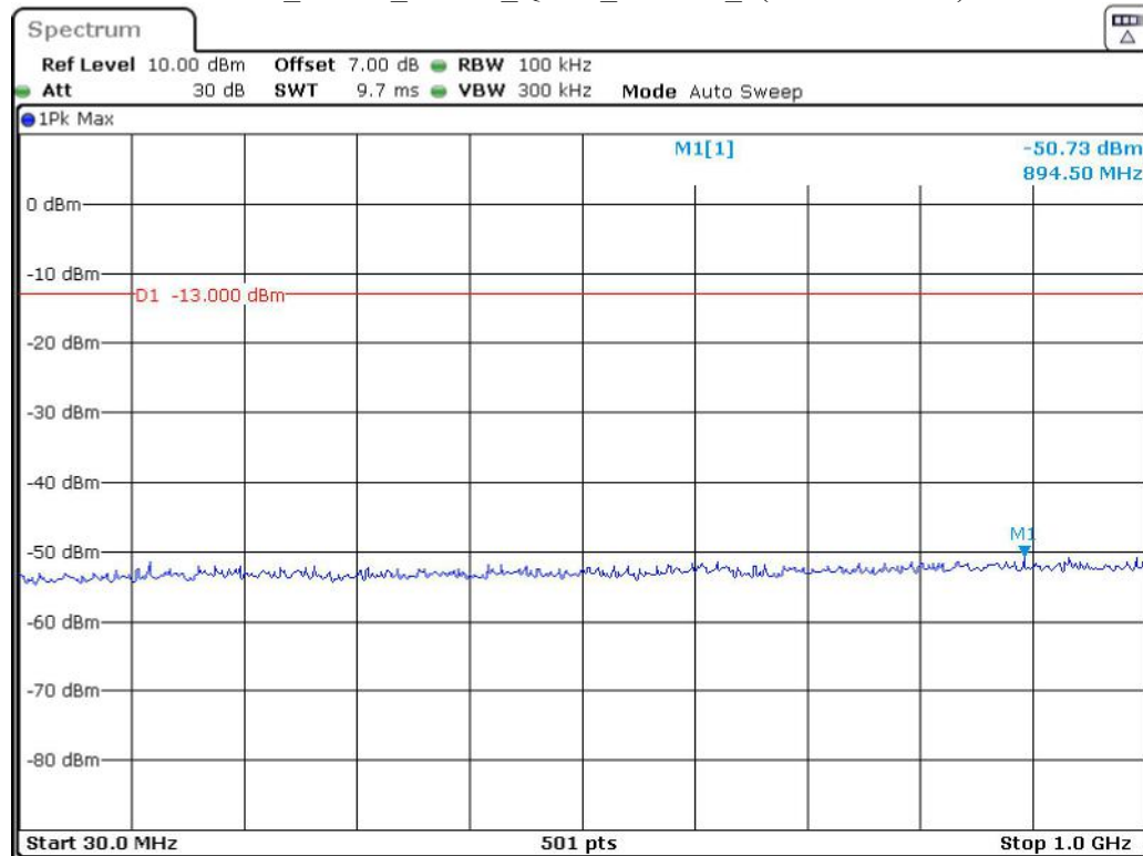
Band 4_5 MHz_Middle_QPSK_RB25#0_1(30MHz-1GHz)
