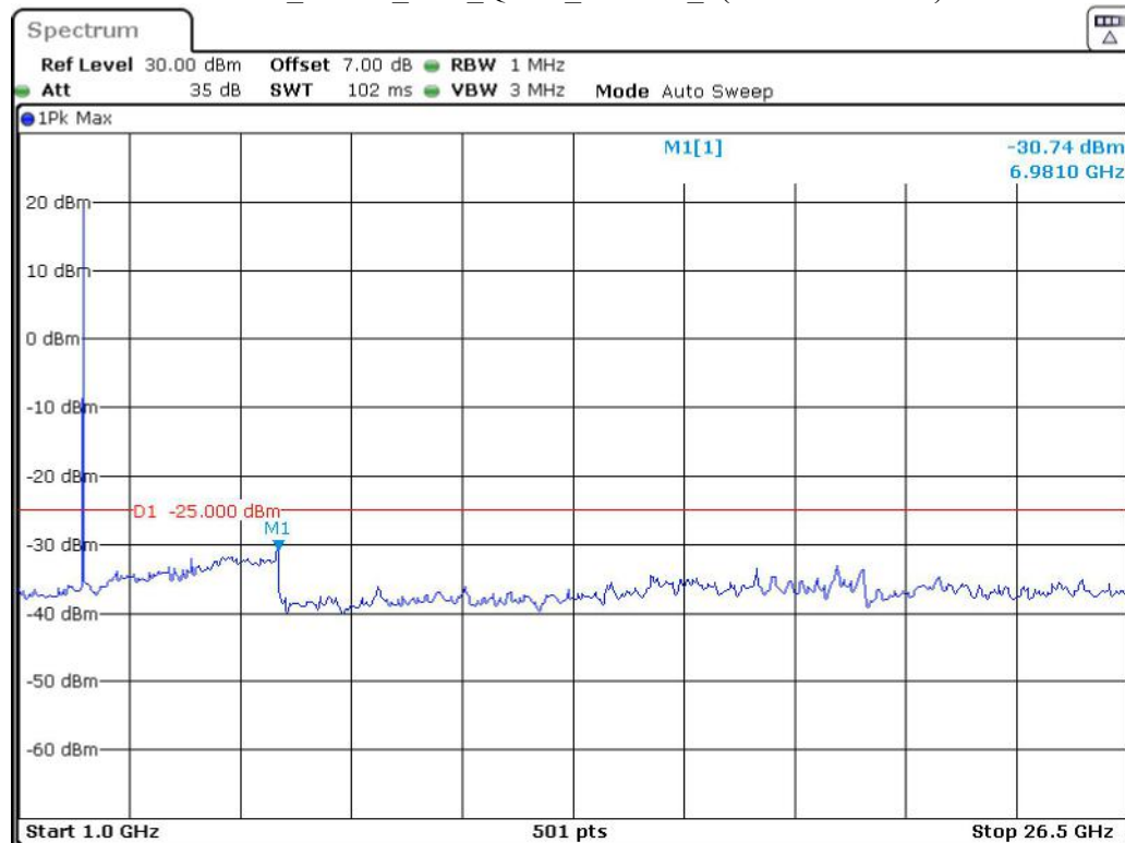
Band 7_5 MHz_Low_QPSK_RB25#0_2(1GHz-26.5GHz)
