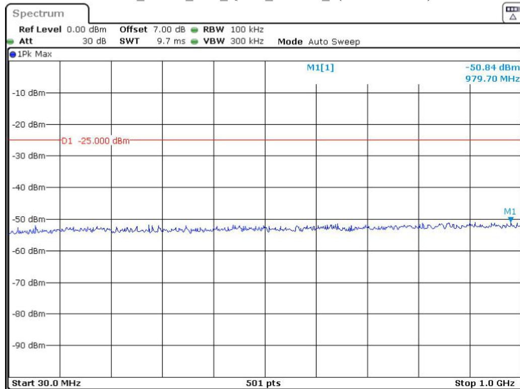
Band 7_5 MHz_Low_QPSK_RB25#0_1(30MHz-1GHz)
