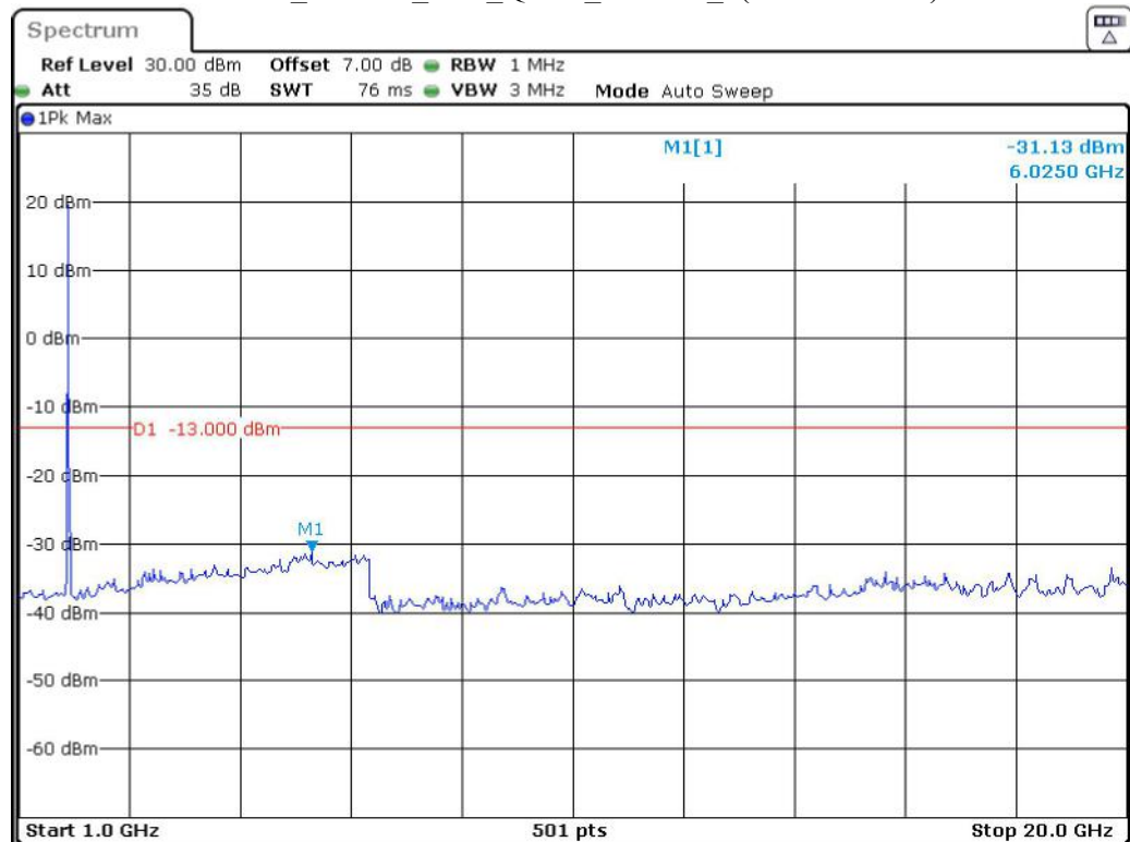
Band 2_15 MHz_Low_QPSK_RB75#0_2(1GHz-20GHz)
