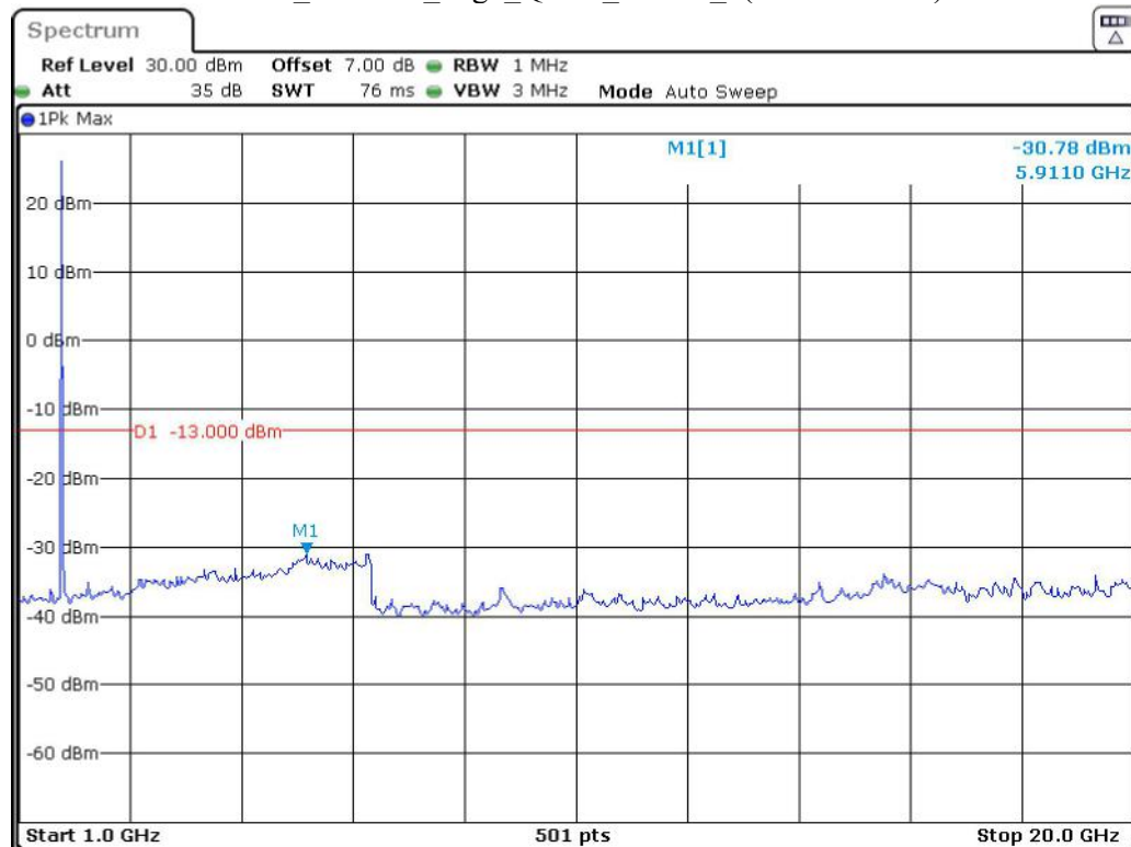
Band 4_1.4 MHz_High_QPSK_RB6#0_2(1GHz-20GHz)
