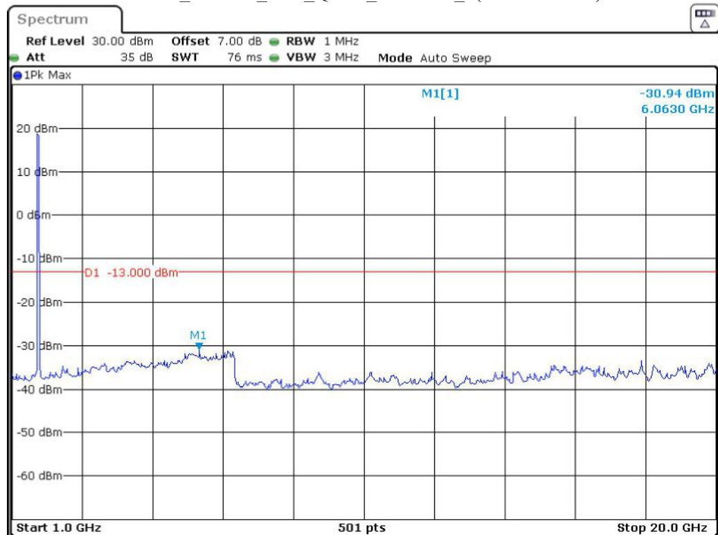
Band 4_20 MHz_Low_QPSK_RB100#0_2(1GHz-20GHz)
