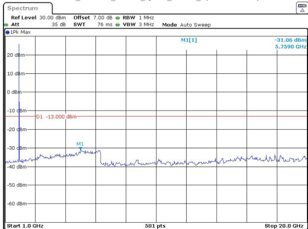
Band 2_1.4 MHz_Middle_QPSK_RB6#0_2(1GHz-20GHz)
