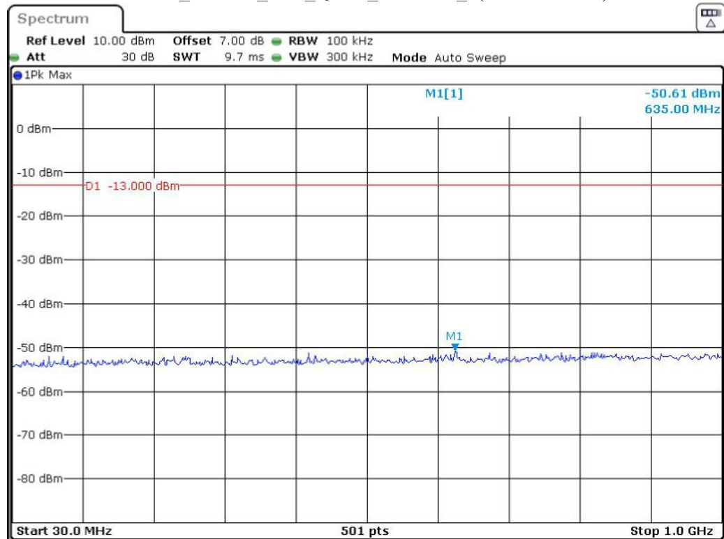
Band 4_20 MHz_Low_QPSK_RB100#0_1(30MHz-1GHz)
