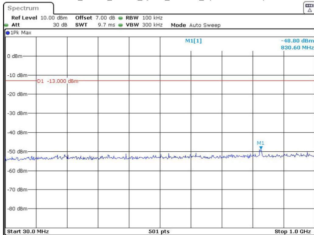
Band 2_5 MHz_Middle_QPSK_RB25#0_1(30MHz-1GHz)
