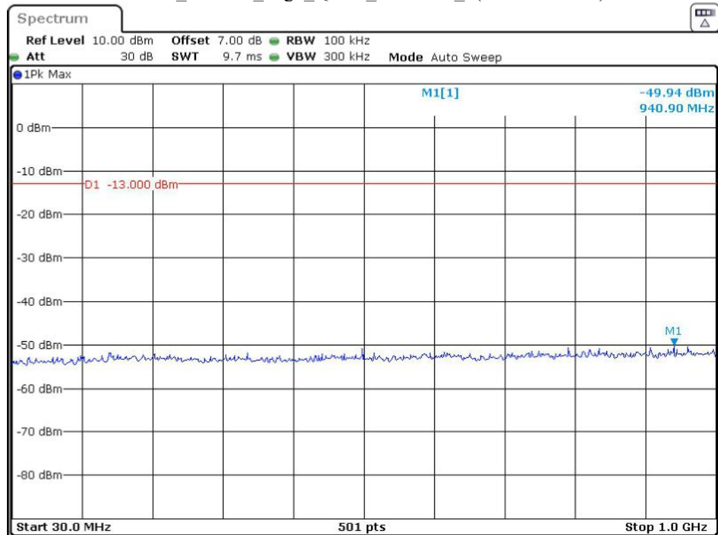
Band 2_20 MHz_High_QPSK_RB100#0_1(30MHz-1GHz)
