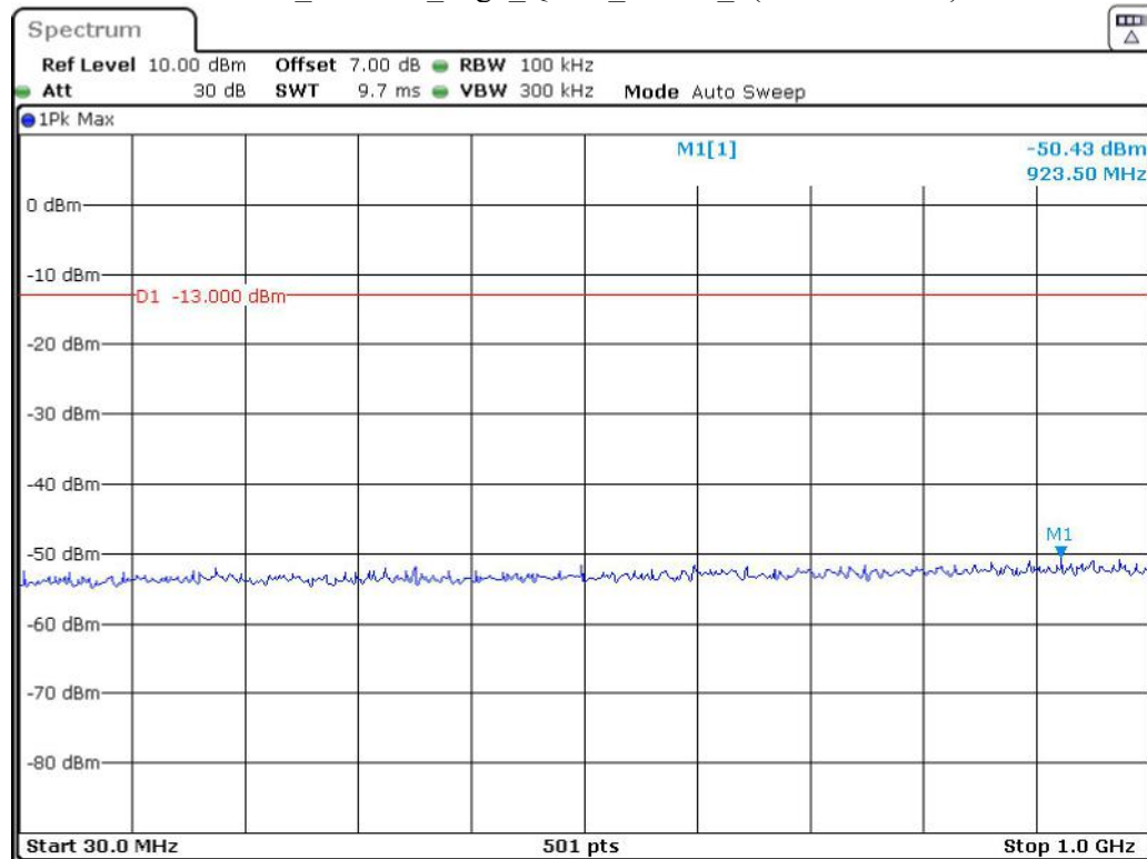
Band 4_1.4 MHz_High_QPSK_RB6#0_1(30MHz-1GHz)
