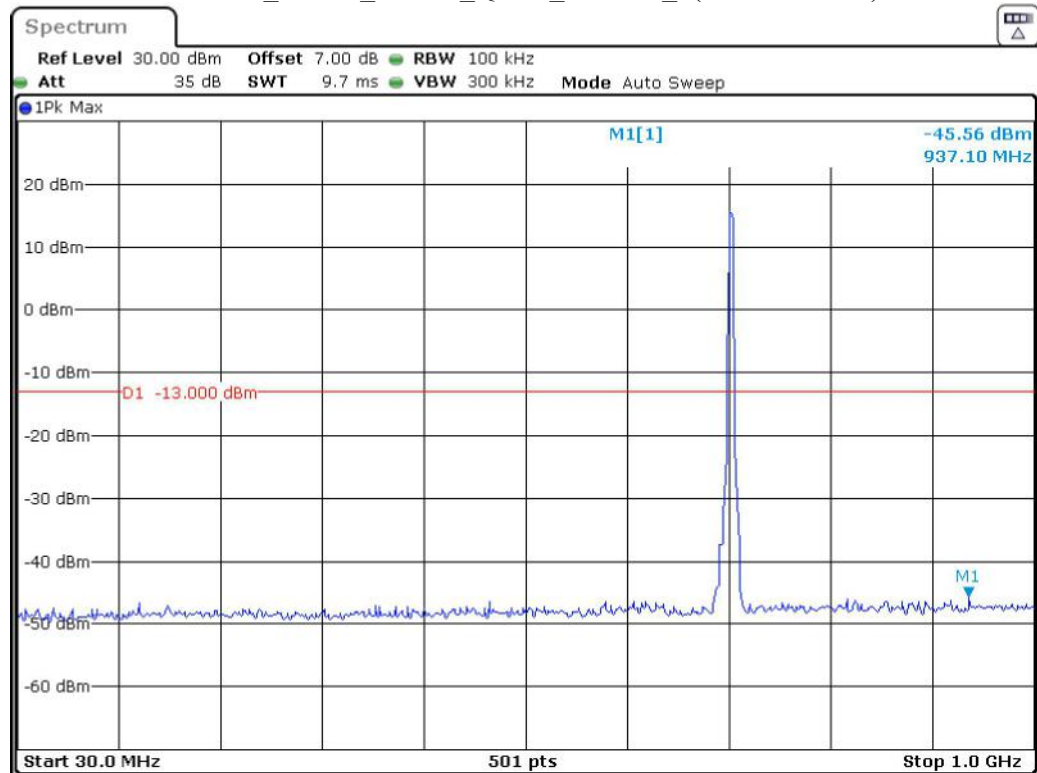
Band 17_5 MHz_Middle_QPSK_RB25#0_1(30MHz-1GHz)
