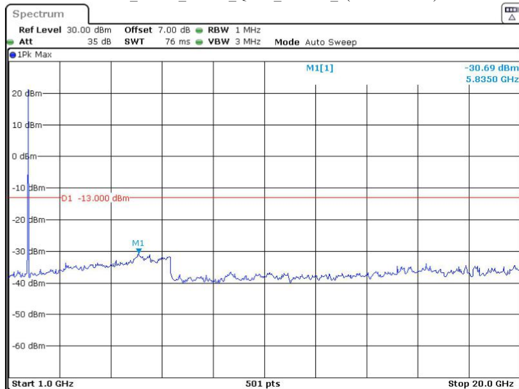
Band 4_5 MHz_Middle_QPSK_RB25#0_2(1GHz-20GHz)
