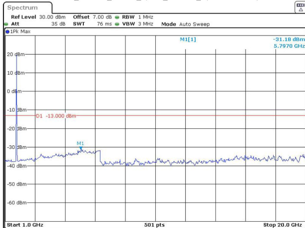
Band 4_15 MHz_Middle_QPSK_RB75#0_2(1GHz-20GHz)
