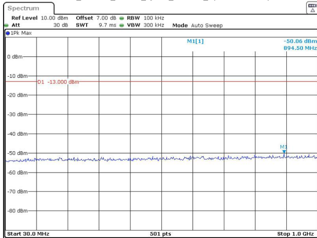
Band 4_15 MHz_Middle_QPSK_RB75#0_1(30MHz-1GHz)
