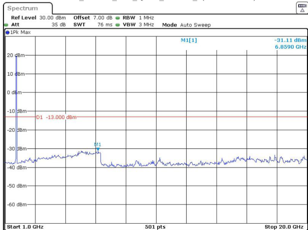
Band 4_15 MHz_Low_QPSK_RB75#0_2(1GHz-20GHz)
