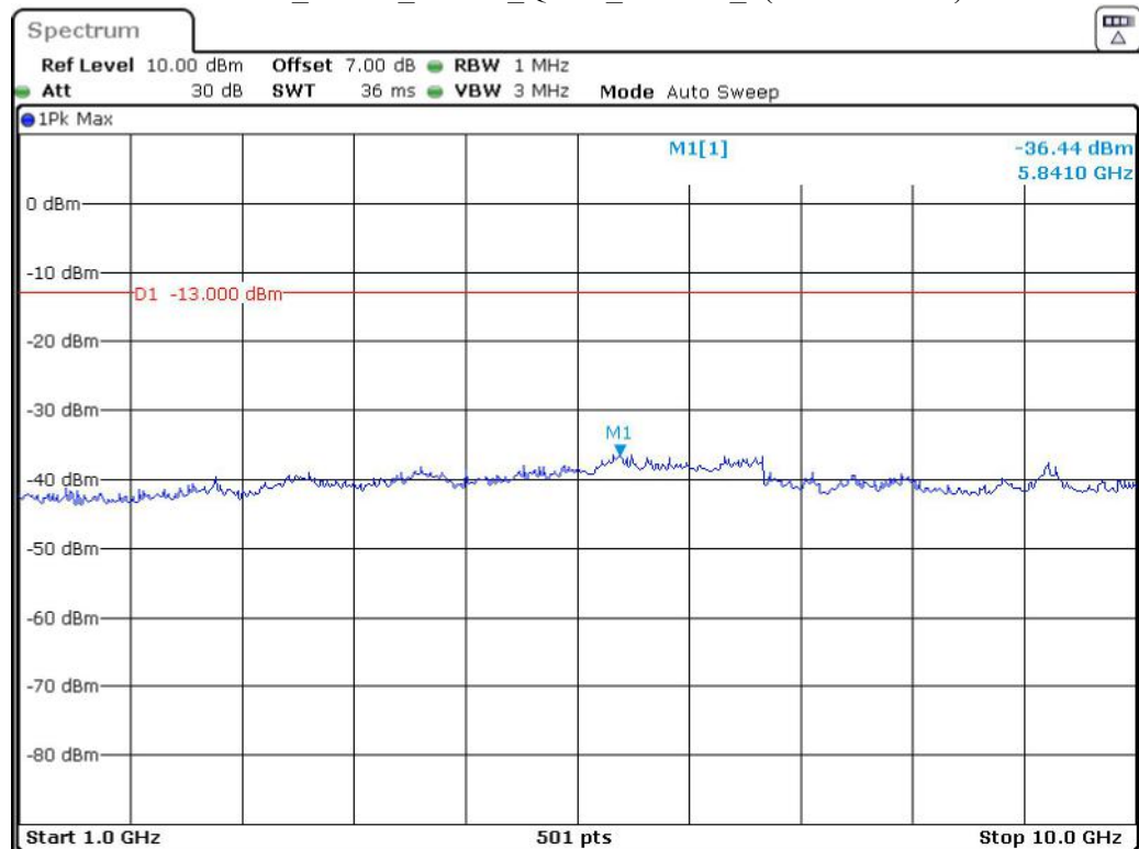
Band 17_5 MHz_Middle_QPSK_RB25#0_2(1GHz-10GHz)
