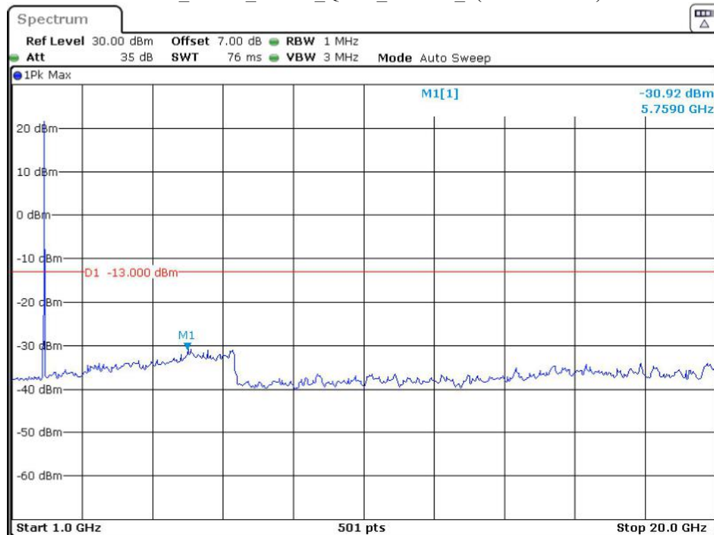
Band 2_5 MHz_Middle_QPSK_RB25#0_2(1GHz-20GHz)
