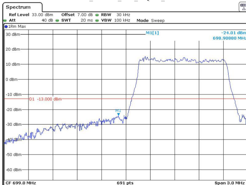
Band 12_1.4 MHz_Low_16QAM_RB6#0
