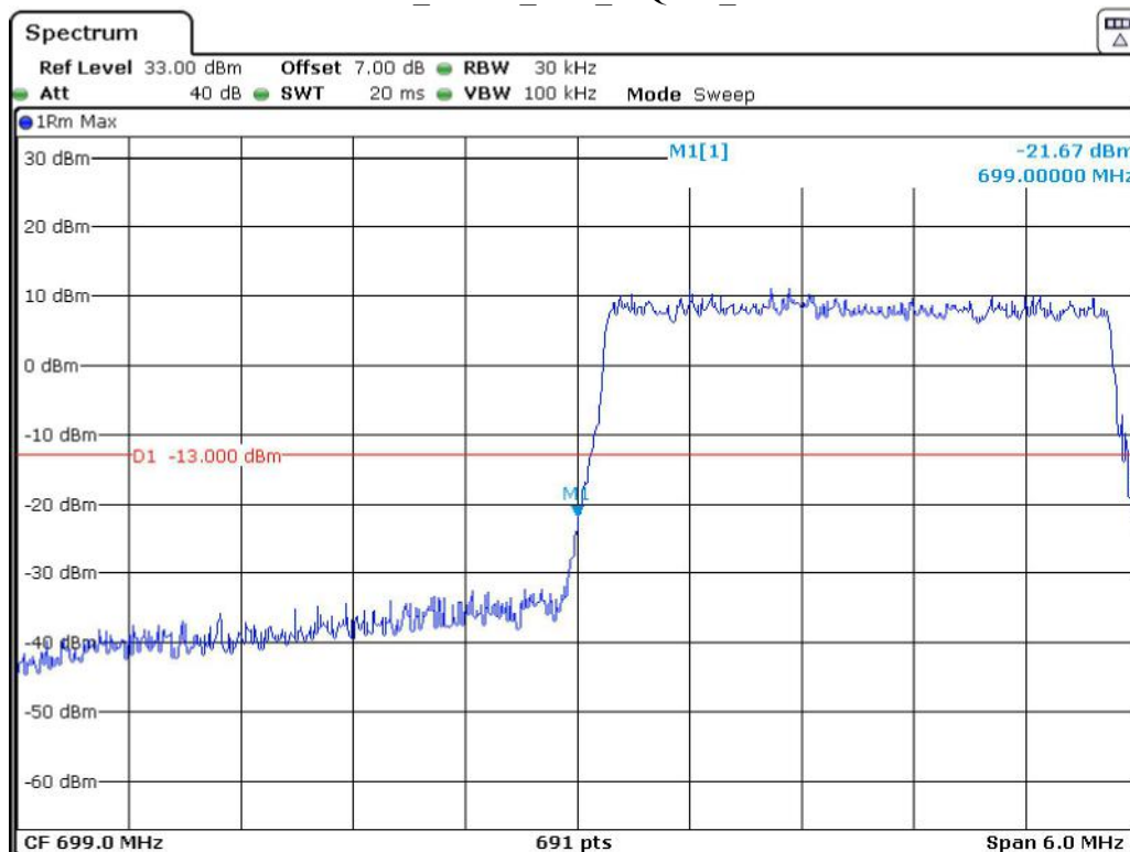
Band 12_3 MHz_Low_16QAM_RB15#0
