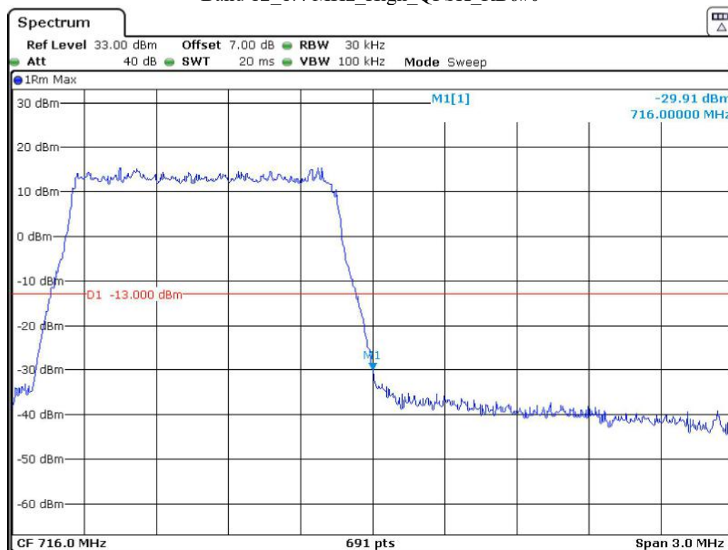
Band 12_1.4 MHz_High_QPSK_RB6#0
