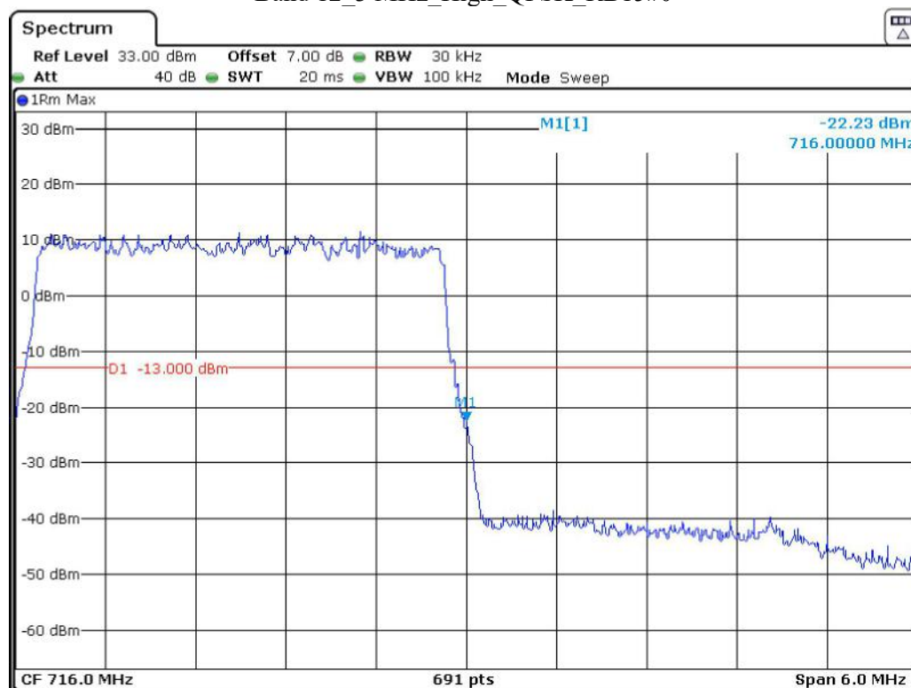
Band 12_3 MHz_High_QPSK_RB15#0
