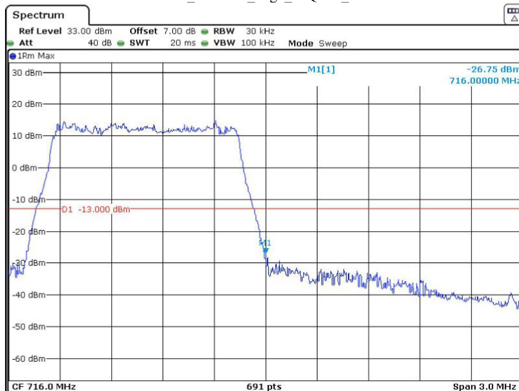
Band 12_1.4 MHz_High_16QAM_RB6#0
