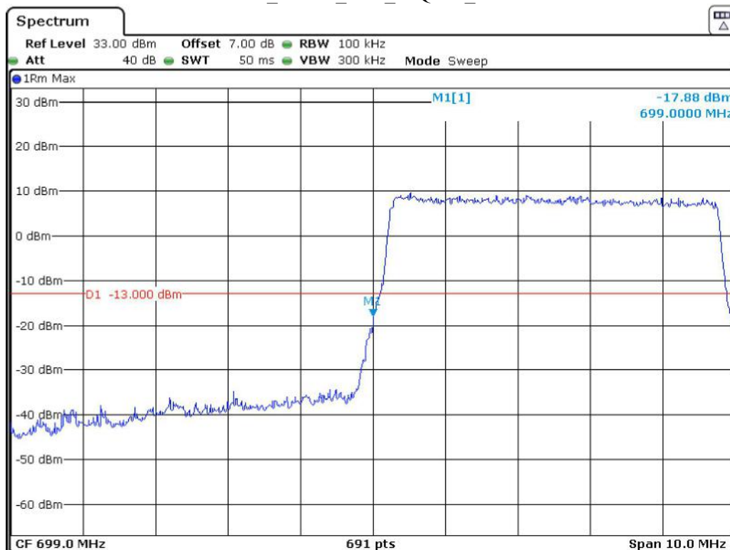
Band 12_5 MHz_Low_16QAM_RB25#0
