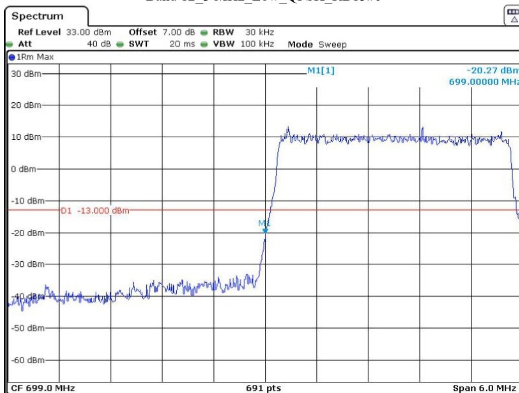
Band 12_3 MHz_Low_QPSK_RB15#0
