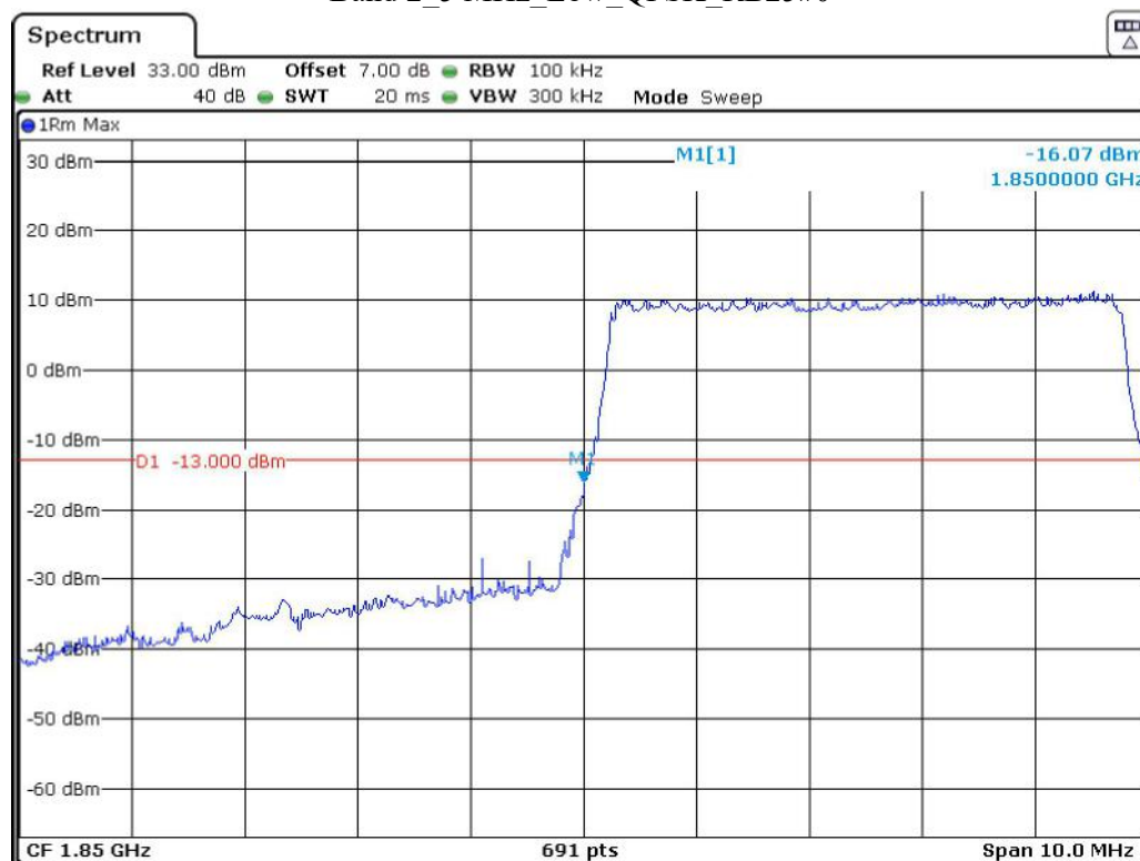
Band 2_5 MHz_Low_QPSK_RB25#0
