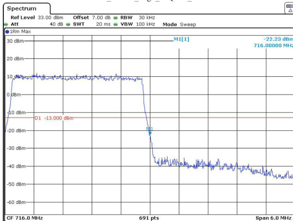
Band 12_3 MHz_High_16QAM_RB15#0
