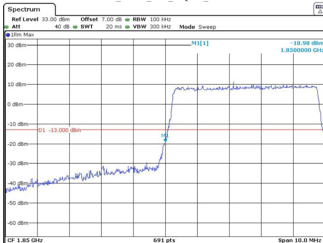
Band 2_5 MHz_Low_16QAM_RB25#0
