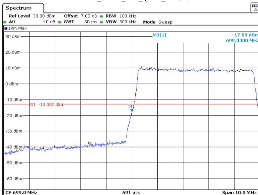
Band 12_5 MHz_Low_QPSK_RB25#0
