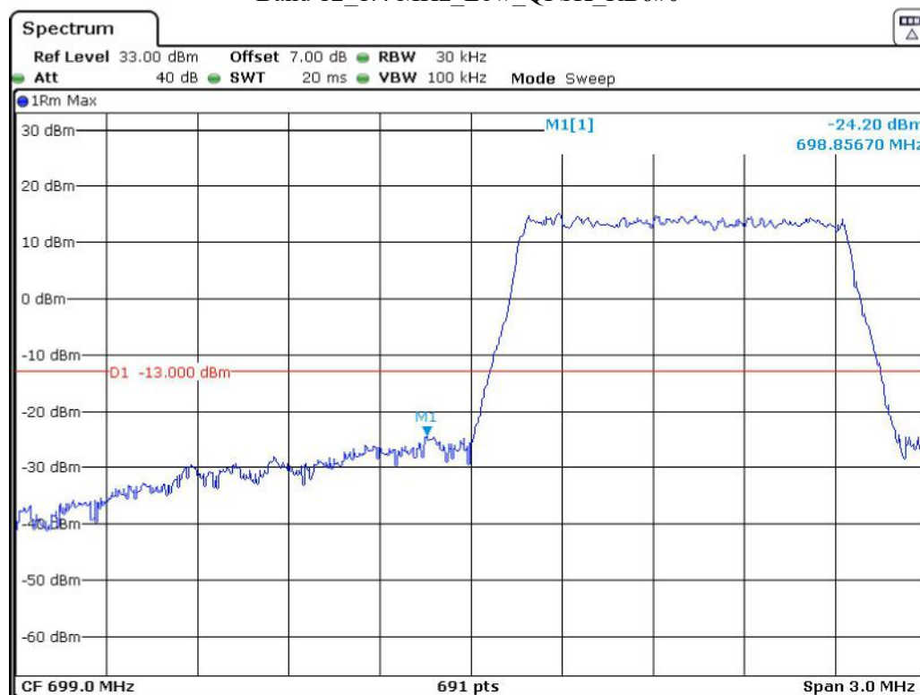
Band 12_1.4 MHz_Low_QPSK_RB6#0
