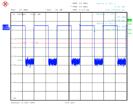
BLE_1M_Low_Channel
