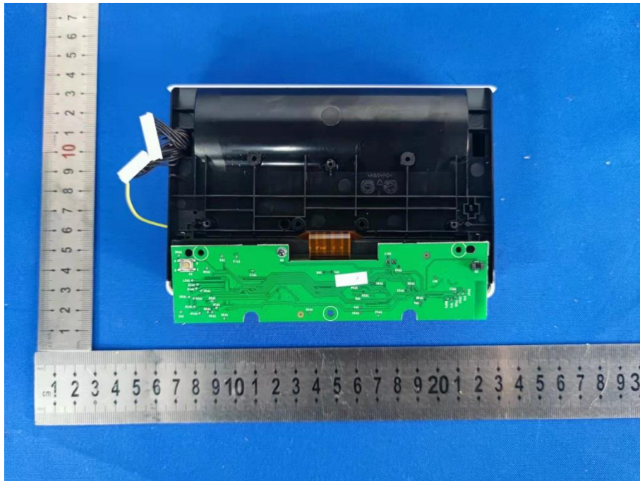
Inside View of Main Board
