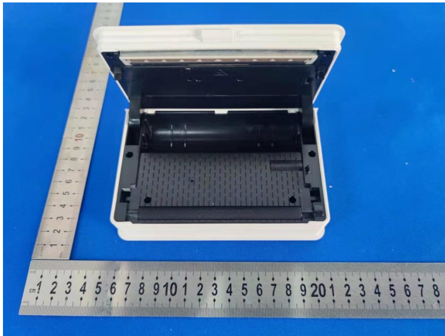
Thermal Paper Compartment View
