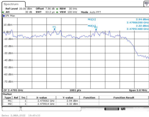
Highest channel
