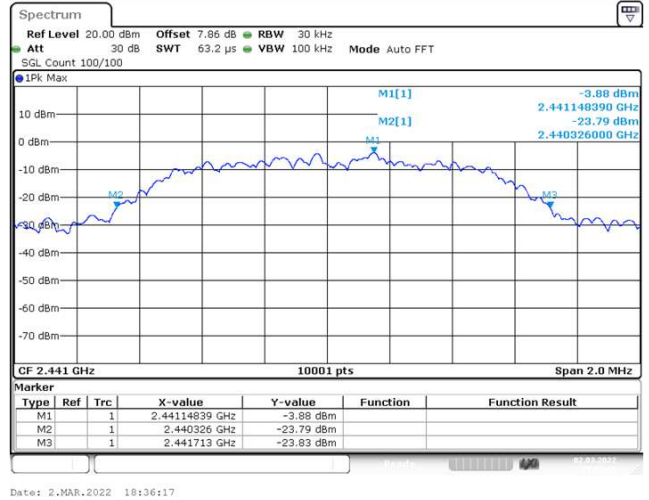
Middle channel
