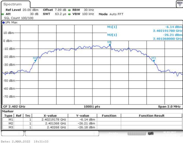
Lowest channel
