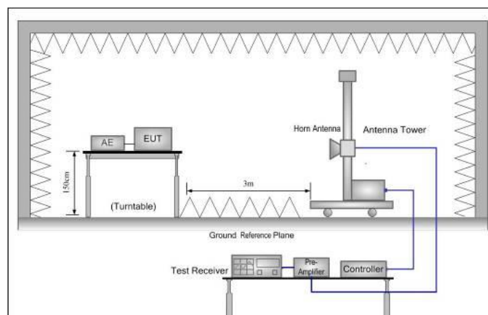
Above 1GHz
