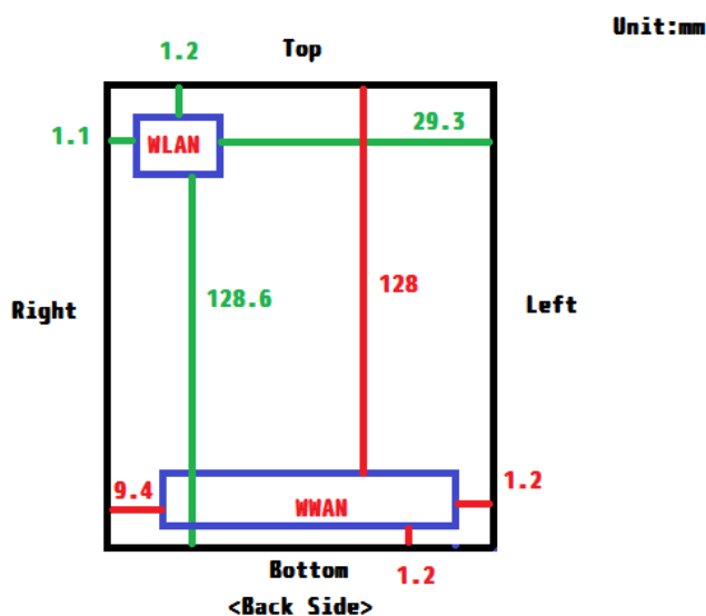
Antenna location
