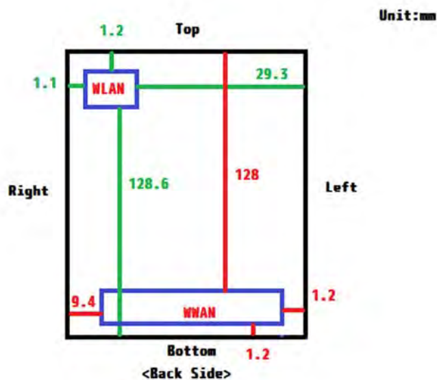
Fig.13 Antenna location
