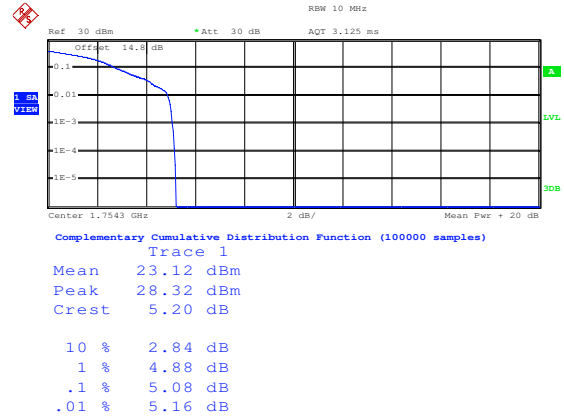
16QAM High channel-1 RB offset 3
