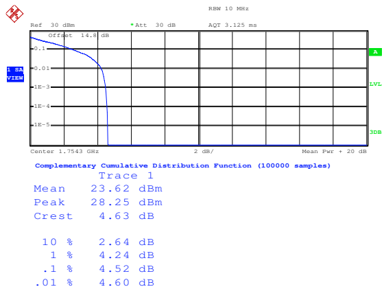
QPSK High channel-1 RB offset 5
