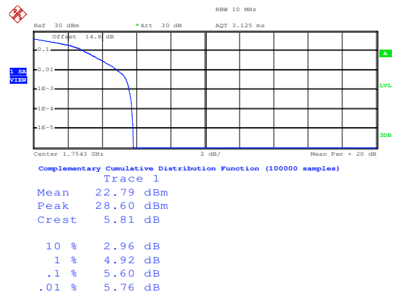
16QAM High channel-3 RB offset 0
