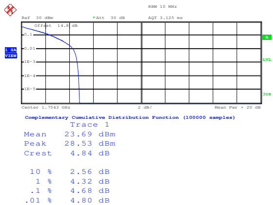
QPSK High channel-3 RB offset 0
