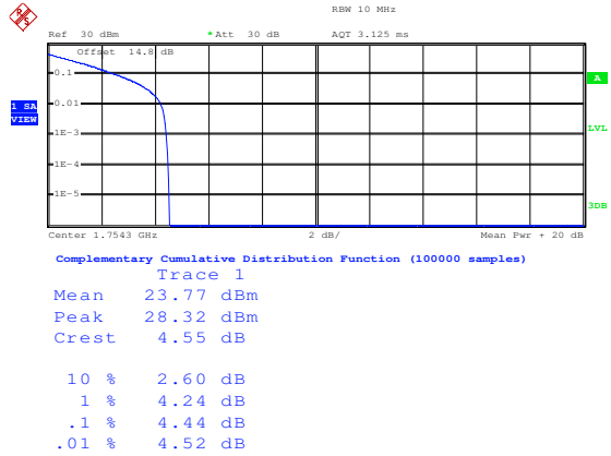
QPSK High channel-1 RB offset 3
