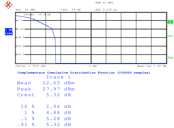
16QAM High channel-1 RB offset 12
