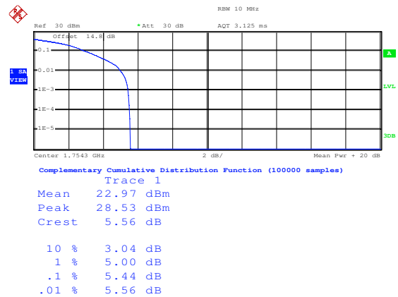
16QAM High channel-1 RB offset 5
