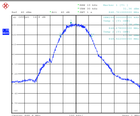
GPRS850-High Channel
