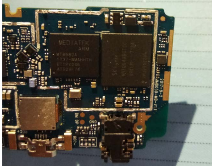
EUT – Main Chip 2 View
