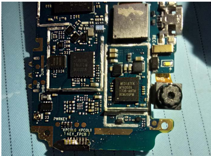
EUT – Main Chip 1 View
