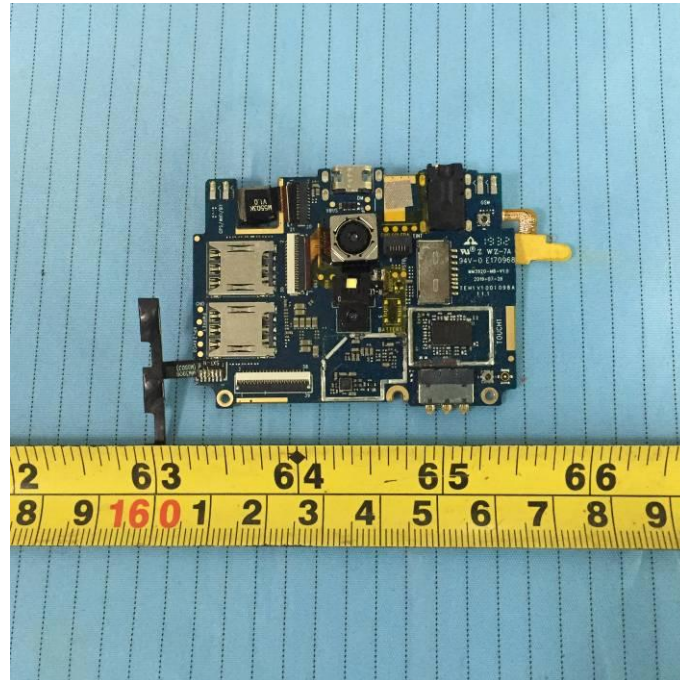
EUT – Main Board Top Shilding off View
