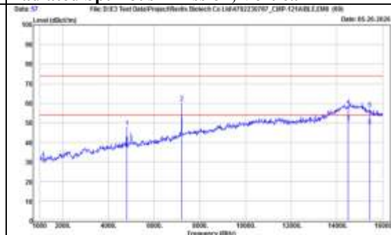
TX, BT-LE-1Mbps - Emission (Ch 0) Radiated Spurious Emission, Vertical
