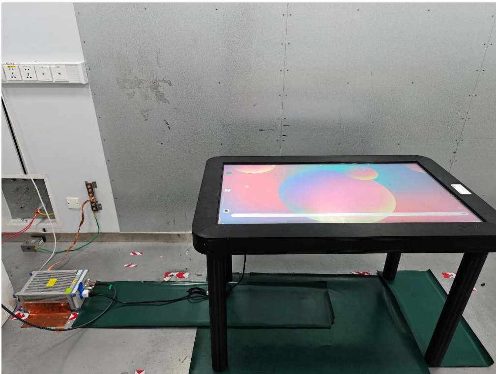
AC CONDUCTED POWER LINE SETUP
