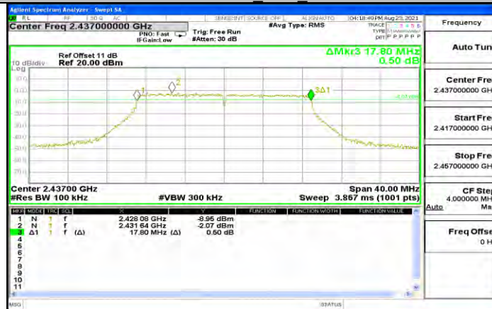
11N20SISO Ant1 2437
