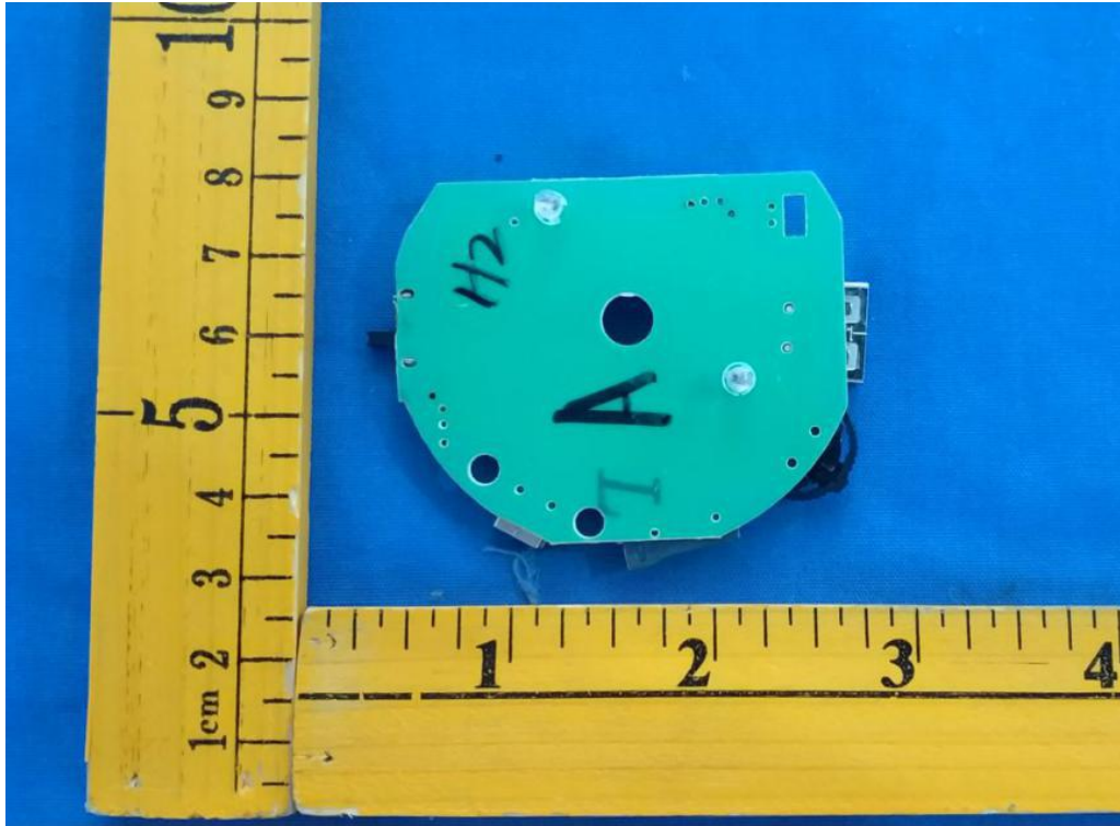
BT:PCB antenna
