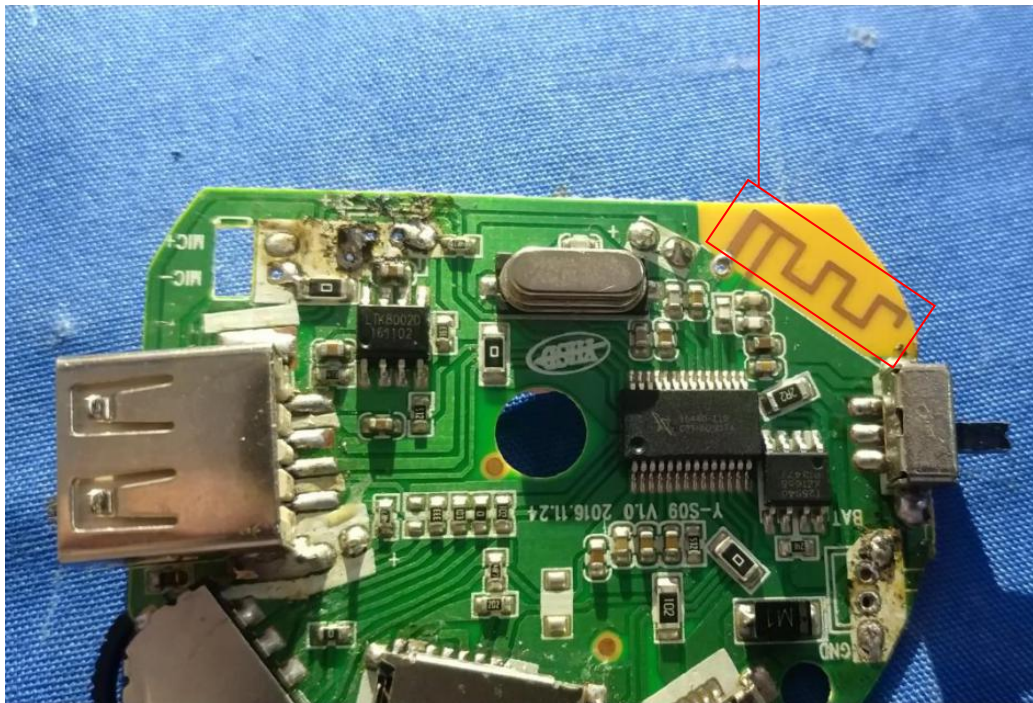
BT:PCB antenna
