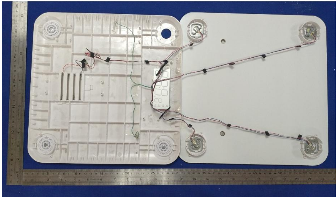
PCB antenna
