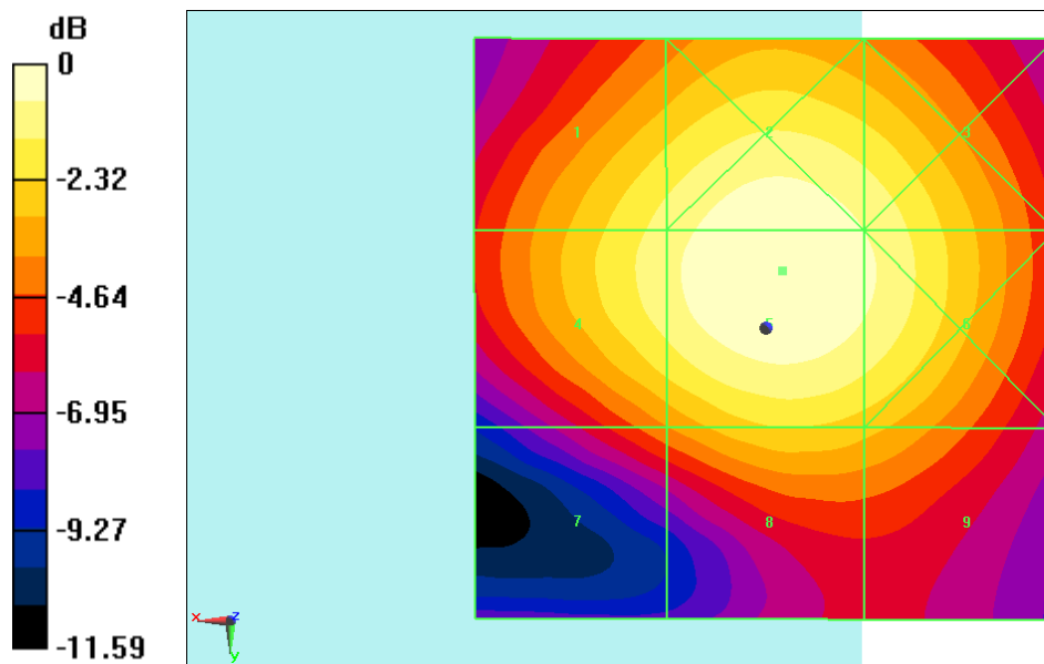
Fig B.5 HAC RF E-Field LTE Band48 QPSK
