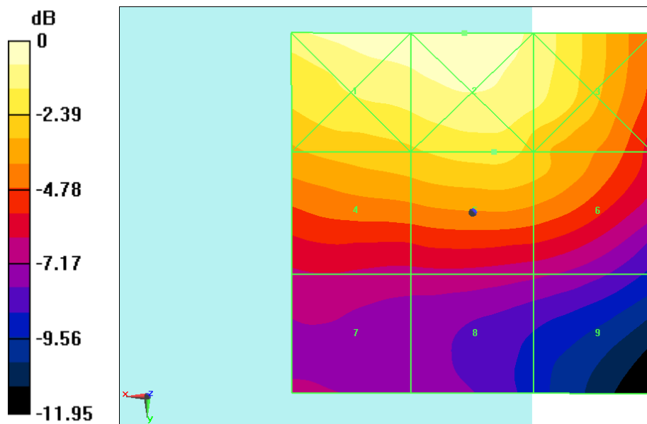
Fig B.4 HAC RF E-Field LTE Band41 PC3 QPSK
