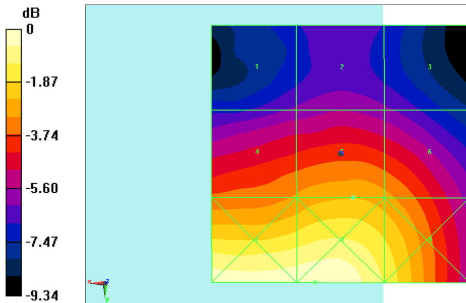
Fig B.6 HAC RF E-Field WIFI2.4G
