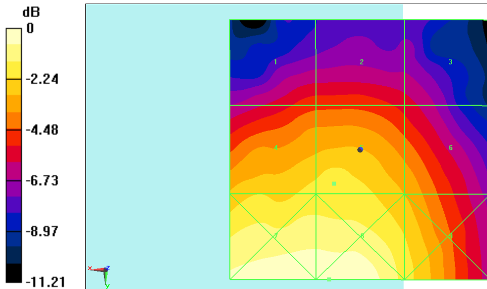
Fig B.4 HAC RF E-Field WIFI2.4G
