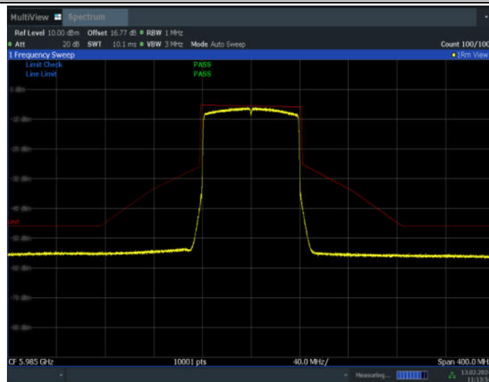
11AX80SISO_Ant7_5985
