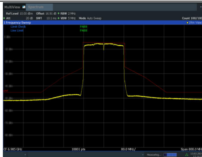
11AX160ISO_Ant7_6985
