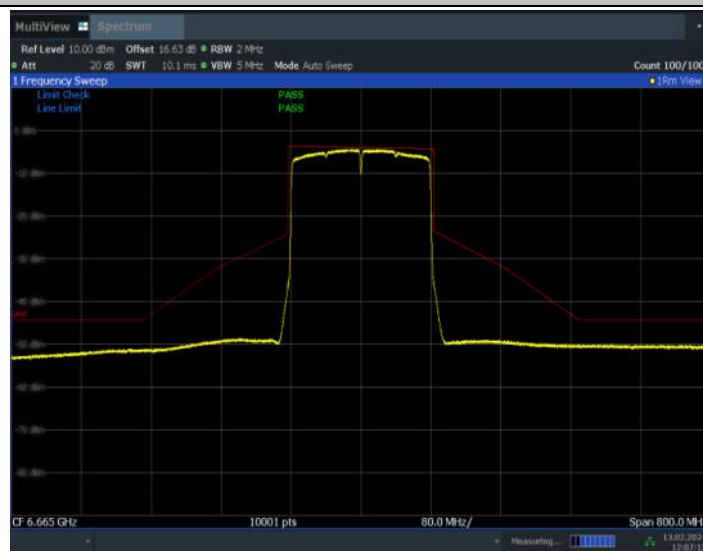
11AX160SISO_Ant7_6665
