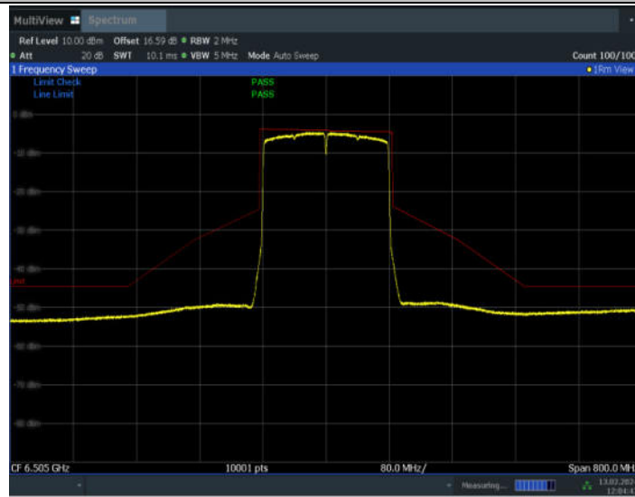
11AX160SISO_Ant7_6505
