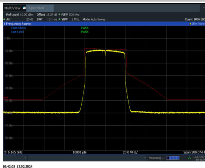
11AX40SISO_Ant7_6165
