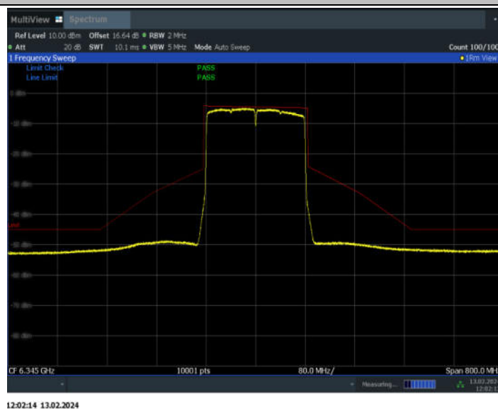
11AX160ISO_Ant7_6345
