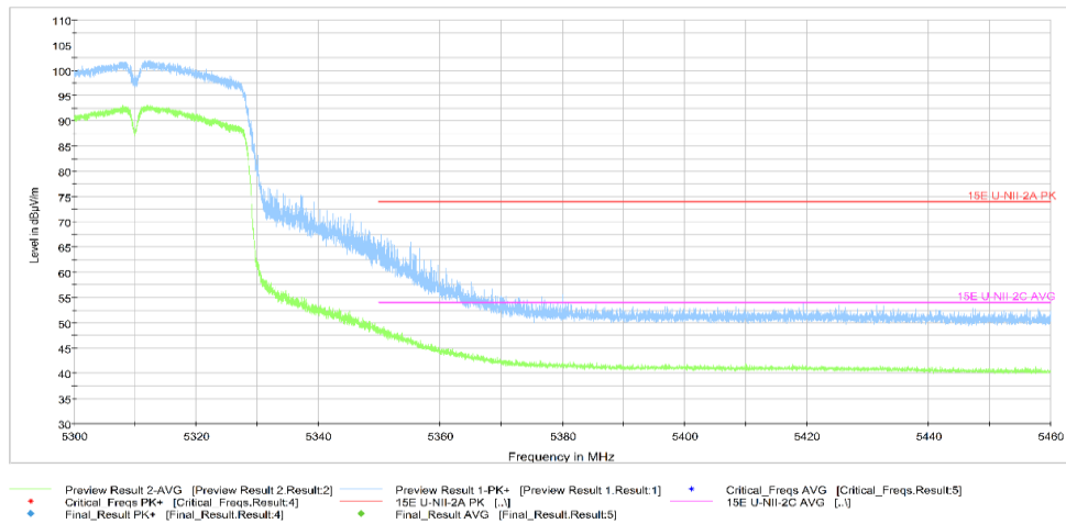
Fig.51 Band Edges (802.11ac-HT40 Ch62, 5310MHz)
