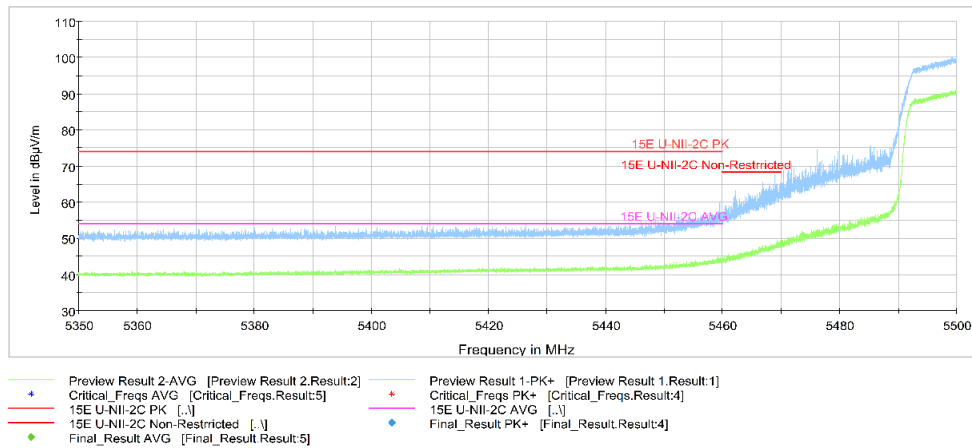
Fig.52 Band Edges (802.11ac-HT40 Ch102, 5510MHz)
