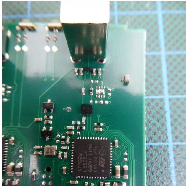
EUT PCB detailed view 3
