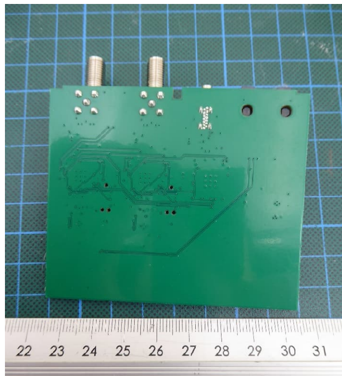
EUT PCB Bottom view
