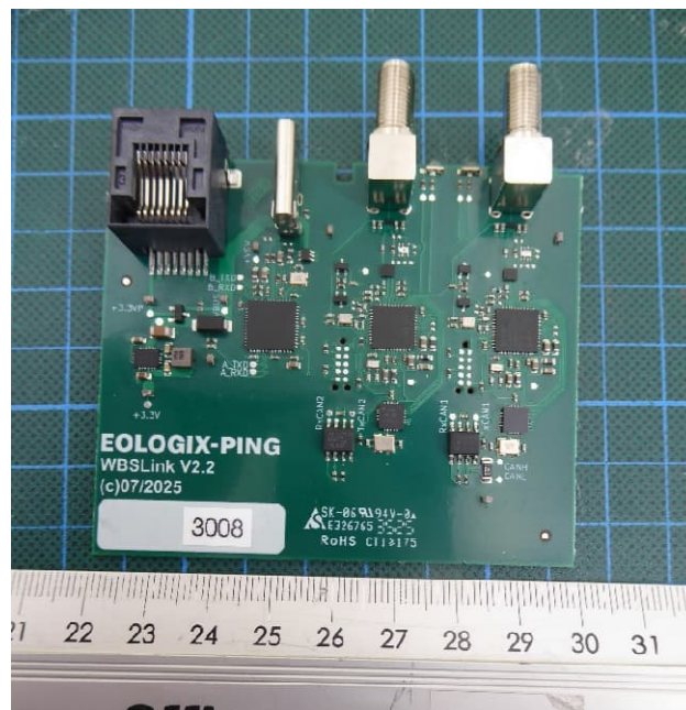
EUT PCB Top view
