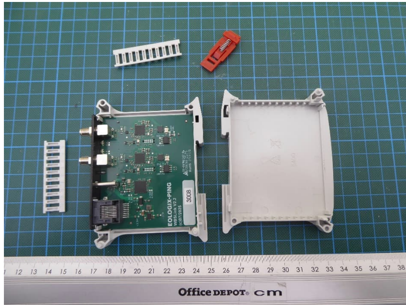
EUT internal view 1
