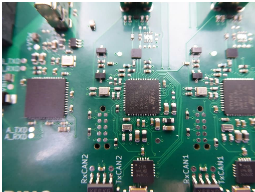
EUT PCB detailed view 2
