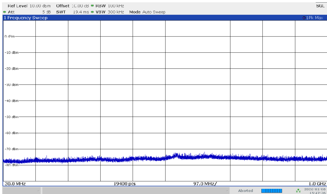
Results from 30 MHz to 1 GHz
