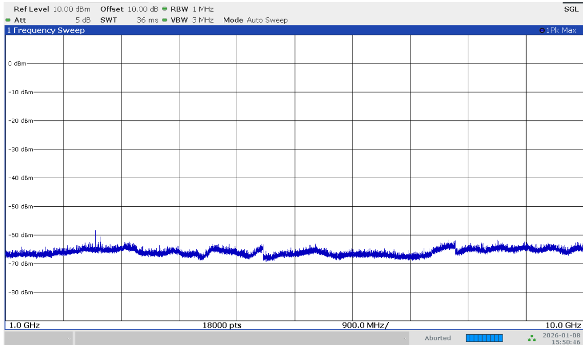
Results from 1 GHz to 10 GHz
