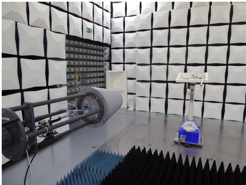
EUT @ 1.50m
