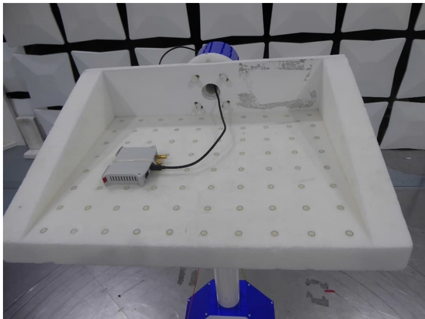
EUT position #1 (setup above 1 GHz)
