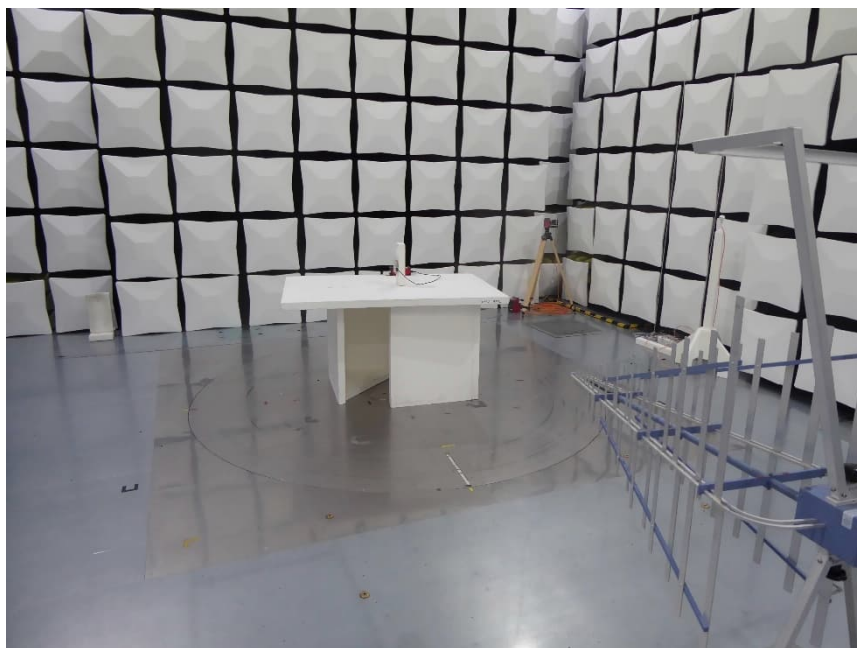
EUT Position #1 Test setup semi-anechoic chamber M276 Preliminary and final measurement
