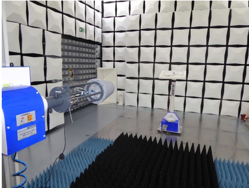
EUT @ 1.50m
