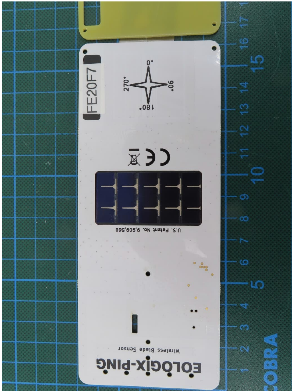
PCB, top view (EUT with SN: FE20F7)
