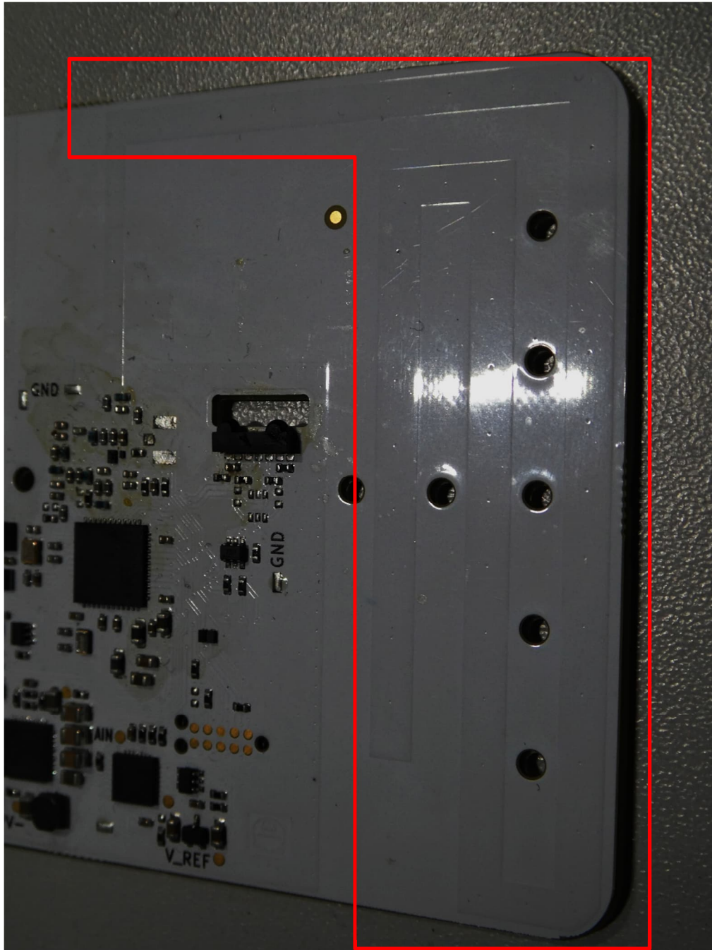
PCB, Antenna structure marked
