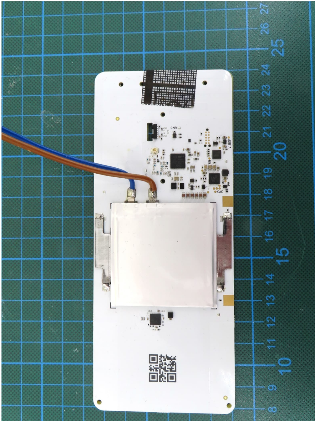
Modified EUT (SN: FE20F8) with temporary antenna connector and external power supply lines
