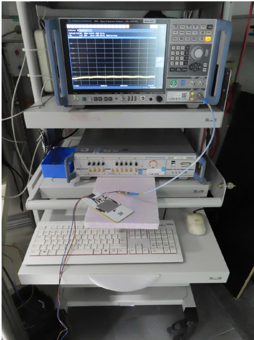
Test setup shielded chamber M4, antenna-port conducted measurements
