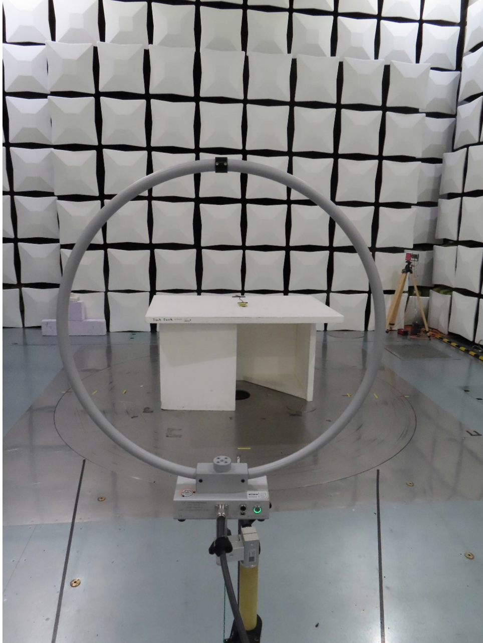
Test setup semi anechoic chamber M276, 9 kHz to 30 MHz
