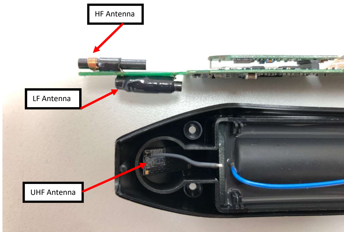
Internal LF, HF and UHF antennas
