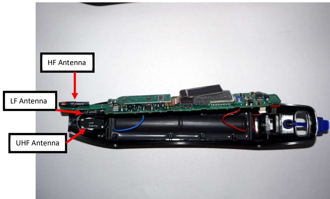
Internal Battery, PCB and antennas
