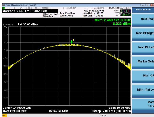
Worst Case Conducted Peak Output Power BLE 500 kbps, 2440 MHz
