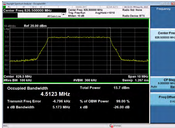
Band5-5MHz-16QAM-20525-25RB#0
