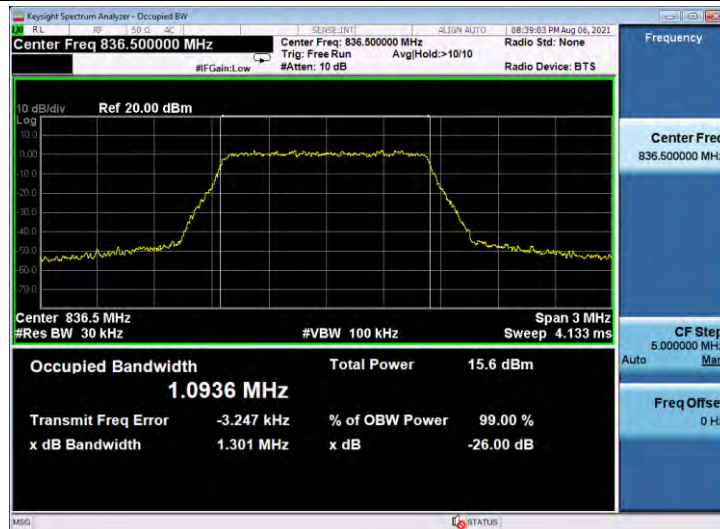
Band5-1.4MHz-QPSK-20643-6RB#0
