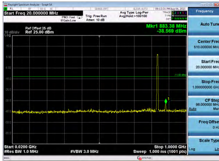
Band5-5MHz-QPSK-20525-25RB#0-Range2:1000~10000MHz
