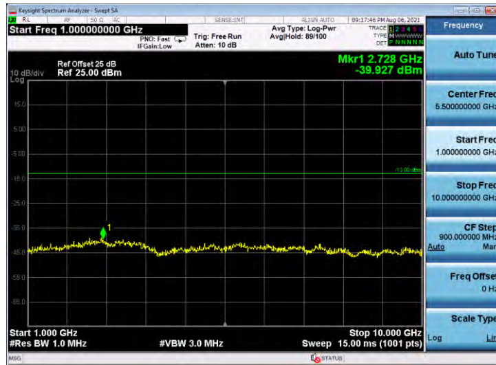
Band5-3MHz-16QAM-20415-15RB#0-Range1:20~1000MHz
