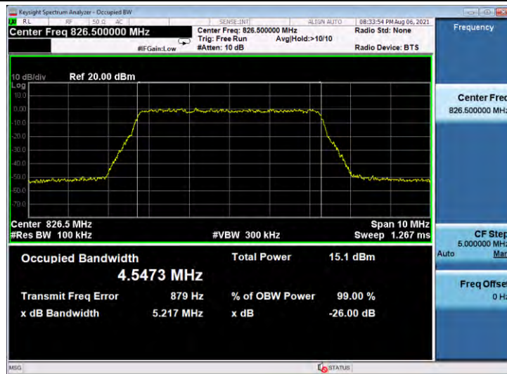
Band5-5MHz-QPSK-20525-25RB#0
