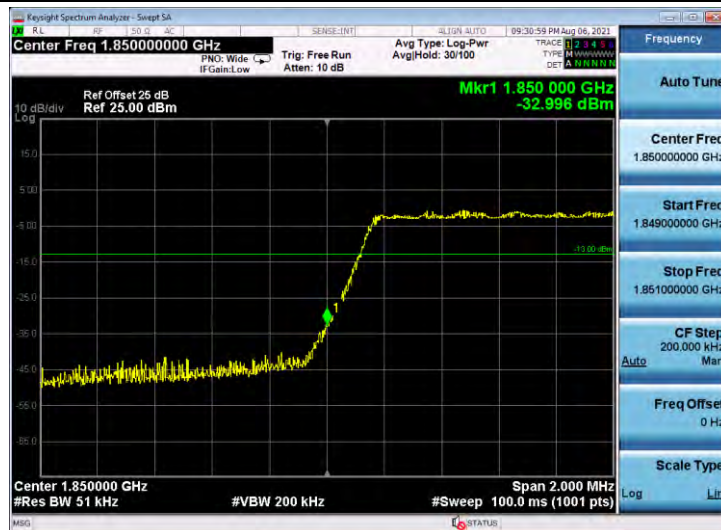
Band2-3MHz-16QAM-19185-15RB#0
