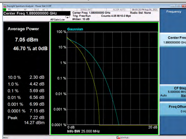
Band2-10MHz-QPSK-19150-50RB#0
