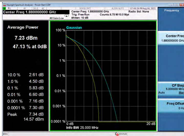
Band2-1.4MHz-16QAM-19193-6RB#0
