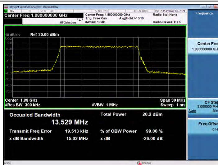
Band2-15MHz-16QAM-19125-75RB#0
