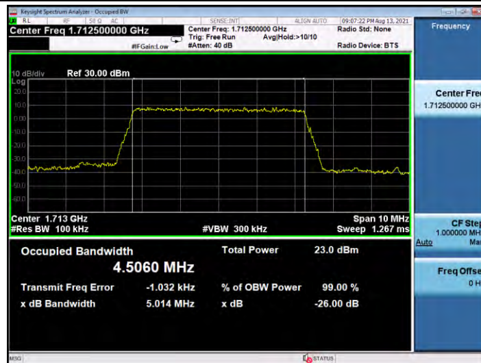
Band4-5MHz-QPSK-20175-25RB#0
