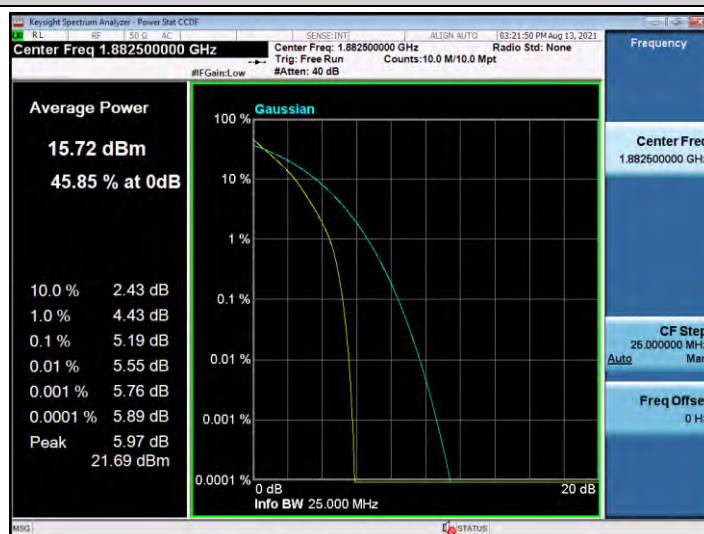
Band25-5MHz-QPSK-26665-25RB#0
