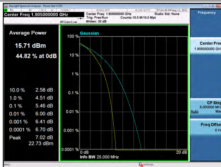
Band25-20MHz-16QAM-26140-100RB#0
