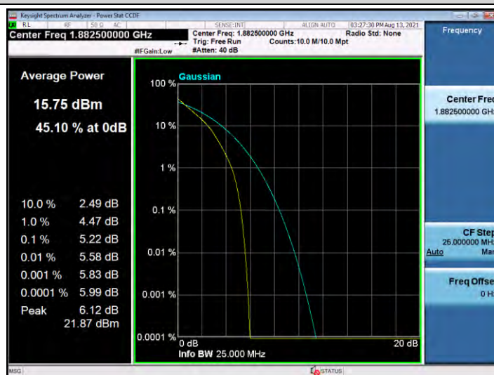
Band25-3MHz-QPSK-26675-15RB#0
