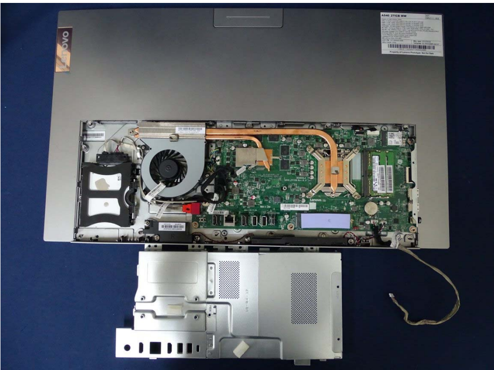
(34) EUT Photo
