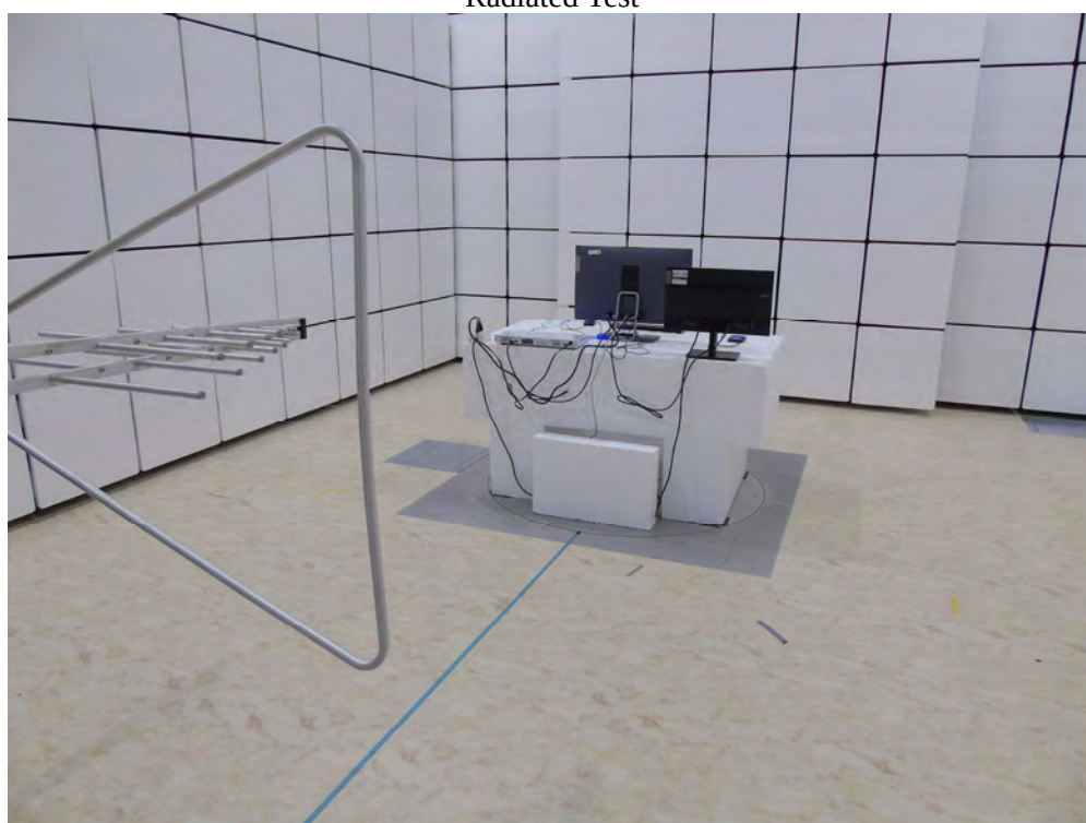
Radiated Test
