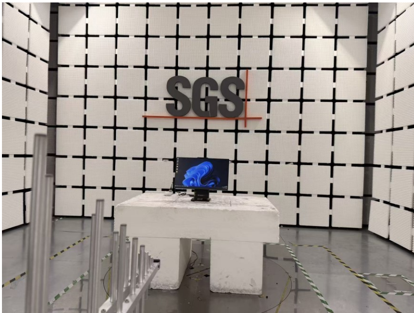
Radiated Test (30MHz-1GHz)
