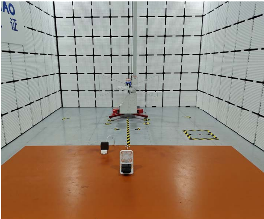
Radiated Emission Above 30MHz
