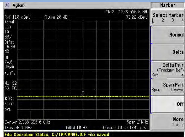
GFSK LOW CHANNEL , AVERAGE
