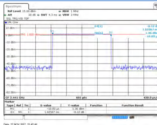
GFSK DH3
