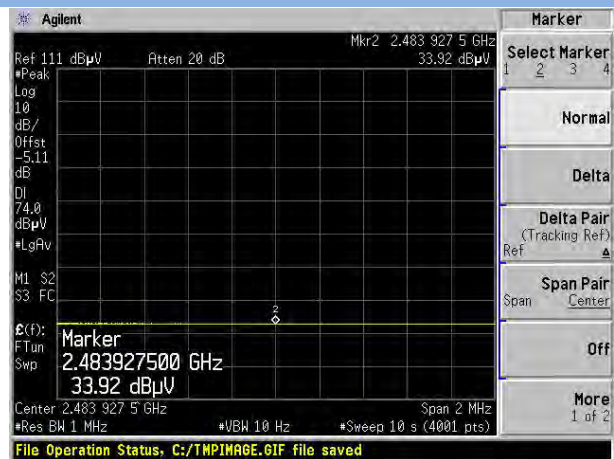
GFSK HIGH CHANNEL , AVERAGE
