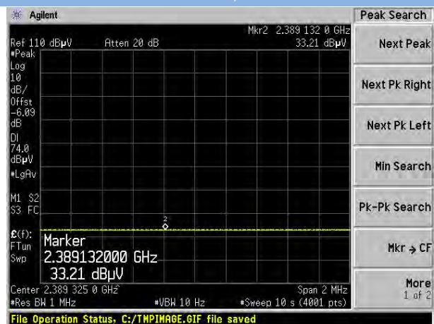
8-DPSK LOW CHANNEL , AVERAGE
