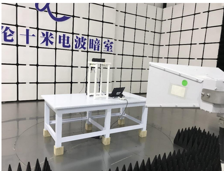
Above 1GHz-BT
