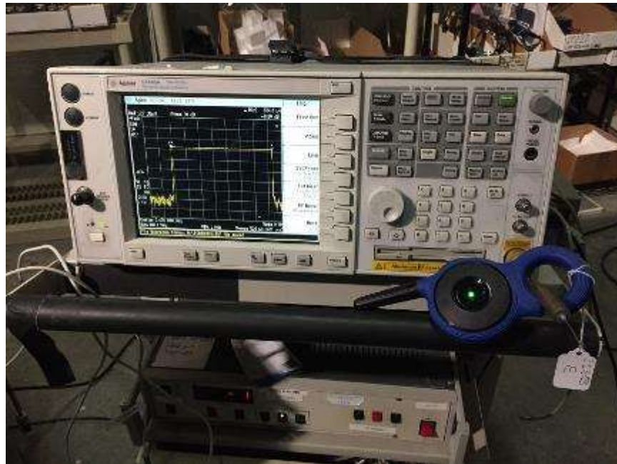
Timing Measurements
